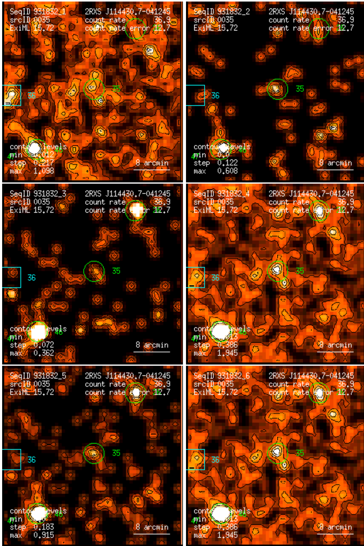
Figure 35: RASS 931832: detection 0035: band rate images, Gaussian filter: (1) PSPC channels 11 – 41, (2) 52 – 90, (3) 91 – 201, (4) 11 – 235, (5) 52 – 201, (6) 11 – 201. Broad band rates in counts/ks. Band rate contour levels in counts/ks/arcmin 2 .
