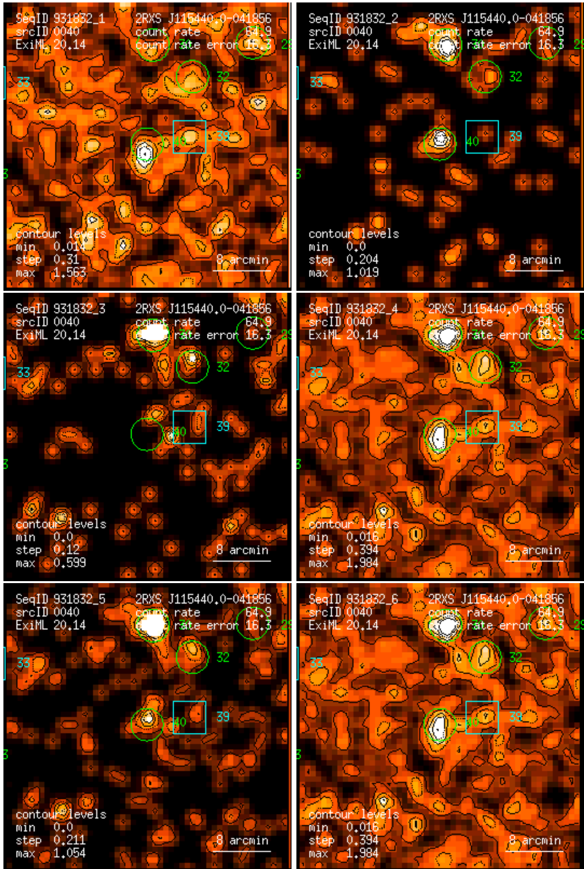
Figure 40: RASS 931832: detection 0040: band rate images, Gaussian filter: (1) PSPC channels 11 – 41, (2) 52 – 90, (3) 91 – 201, (4) 11 – 235, (5) 52 – 201, (6) 11 – 201. Broad band rates in counts/ks. Band rate contour levels in counts/ks/arcmin 2 .
