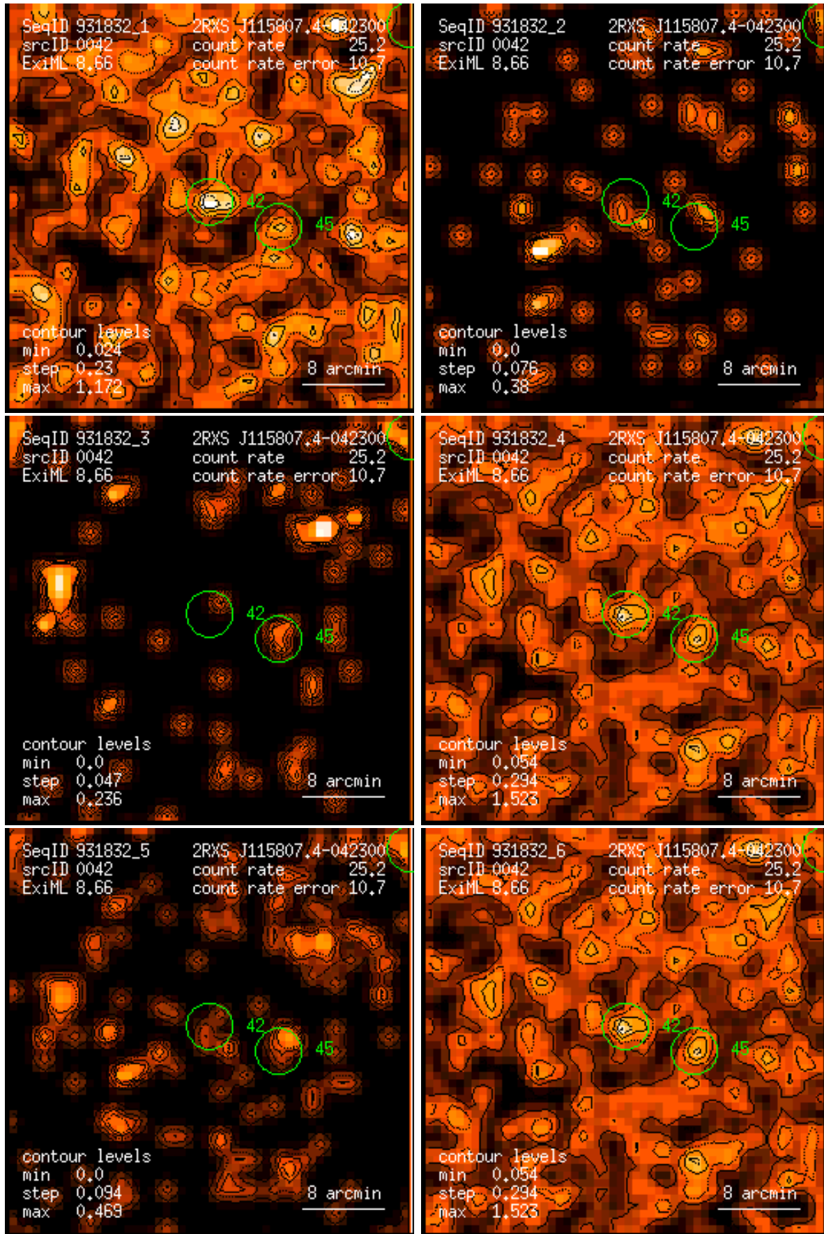
Figure 42: RASS 931832: detection 0042: band rate images, Gaussian filter: (1) PSPC channels 11 – 41, (2) 52 – 90, (3) 91 – 201, (4) 11 – 235, (5) 52 – 201, (6) 11 – 201. Broad band rates in counts/ks. Band rate contour levels in counts/ks/arcmin 2 .
