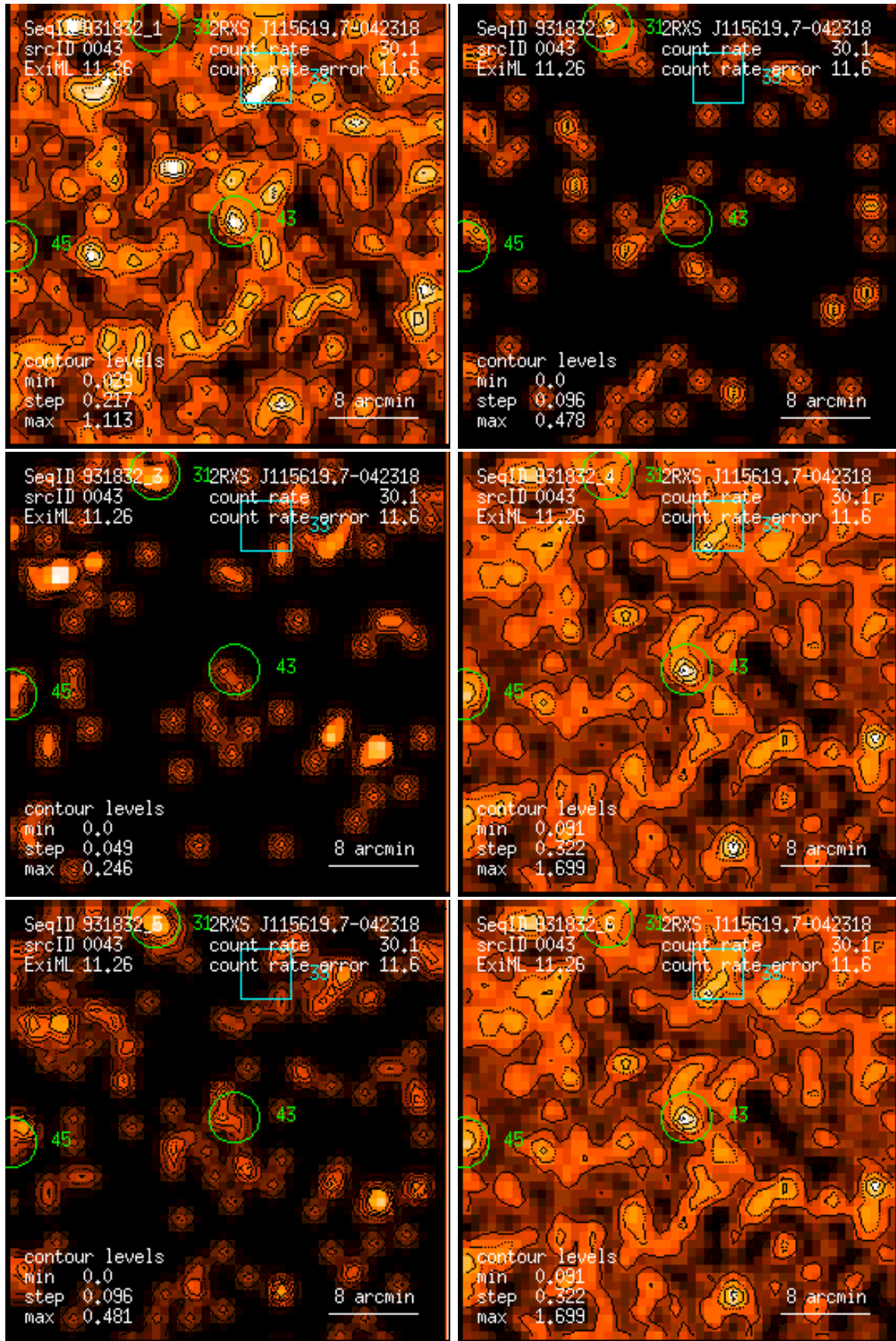
Figure 43: RASS 931832: detection 0043: band rate images, Gaussian filter: (1) PSPC channels 11 – 41, (2) 52 – 90, (3) 91 – 201, (4) 11 – 235, (5) 52 – 201, (6) 11 – 201. Broad band rates in counts/ks. Band rate contour levels in counts/ks/arcmin 2 .
