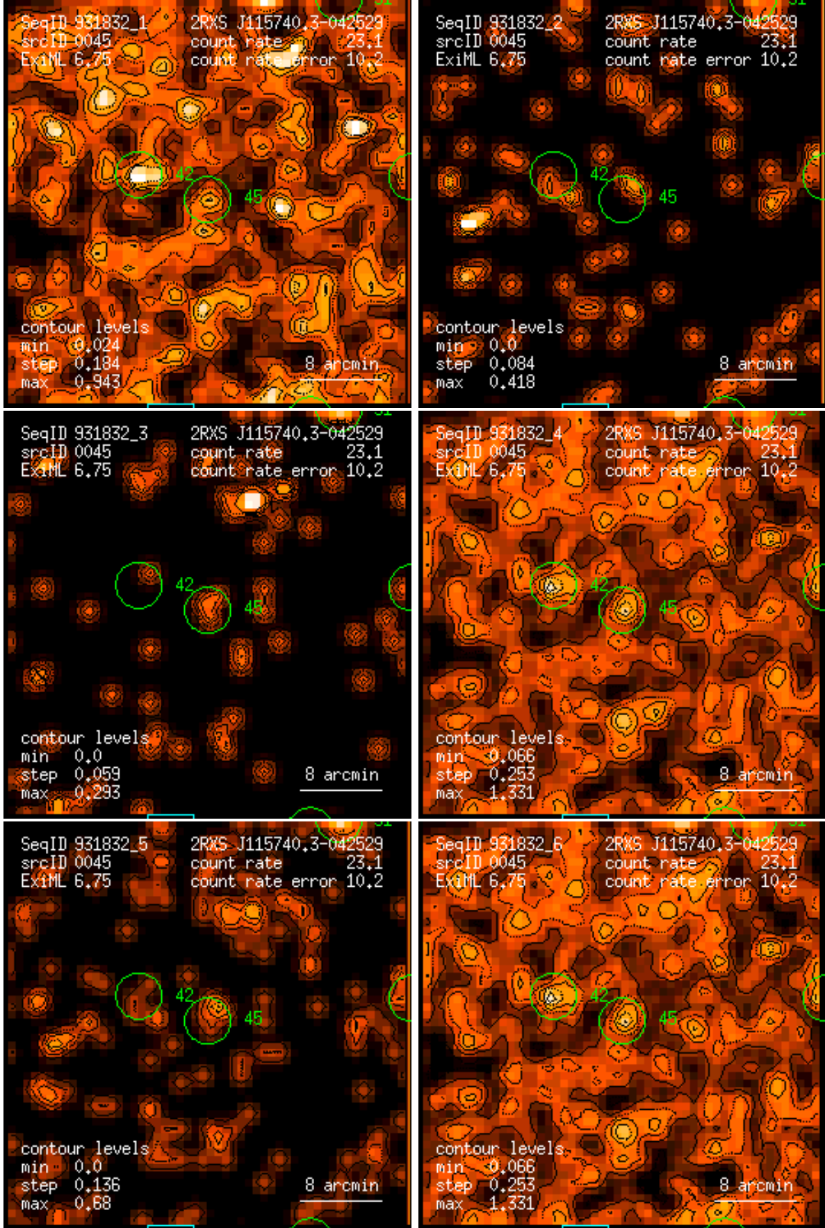
Figure 45: RASS 931832: detection 0045: band rate images, Gaussian filter: (1) PSPC channels 11 – 41, (2) 52 – 90, (3) 91 – 201, (4) 11 – 235, (5) 52 – 201, (6) 11 – 201. Broad band rates in counts/ks. Band rate contour levels in counts/ks/arcmin 2 .
