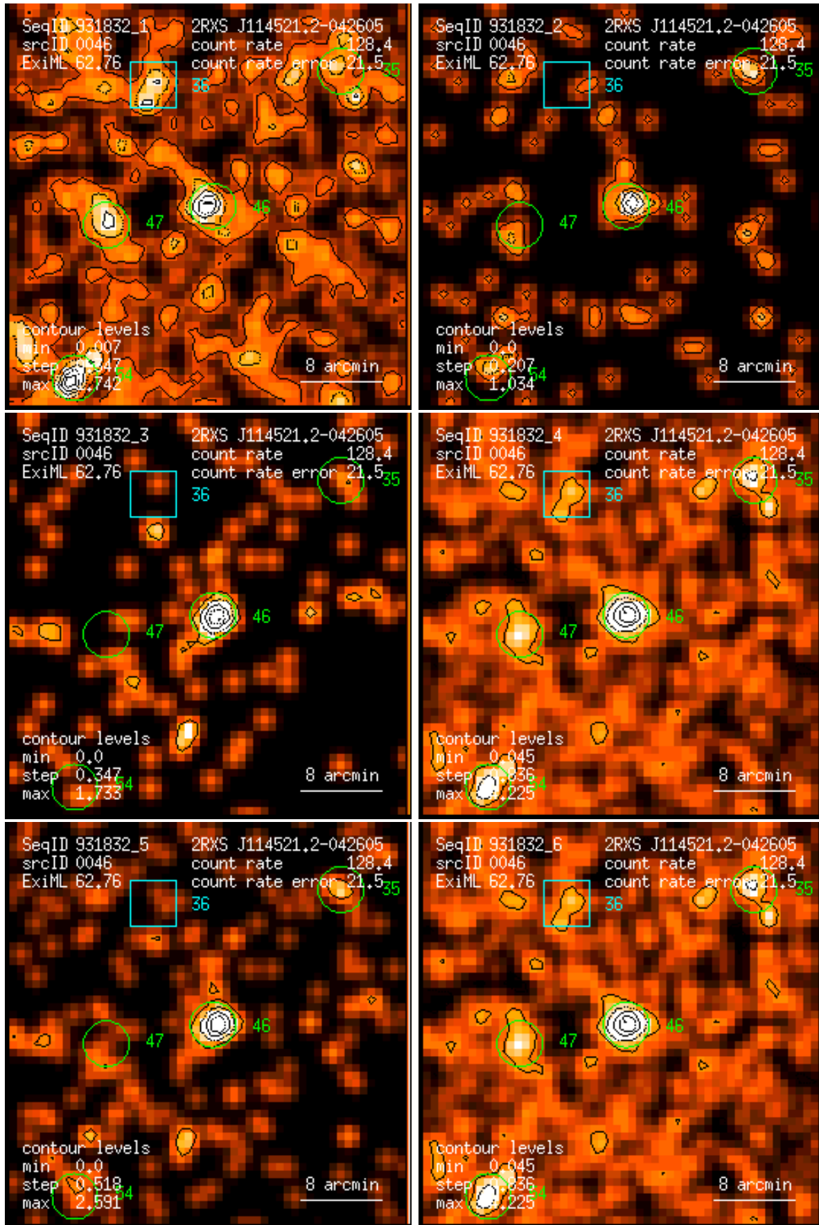
Figure 46: RASS 931832: detection 0046: band rate images, Gaussian filter: (1) PSPC channels 11 – 41, (2) 52 – 90, (3) 91 – 201, (4) 11 – 235, (5) 52 – 201, (6) 11 – 201. Broad band rates in counts/ks. Band rate contour levels in counts/ks/arcmin 2 .
