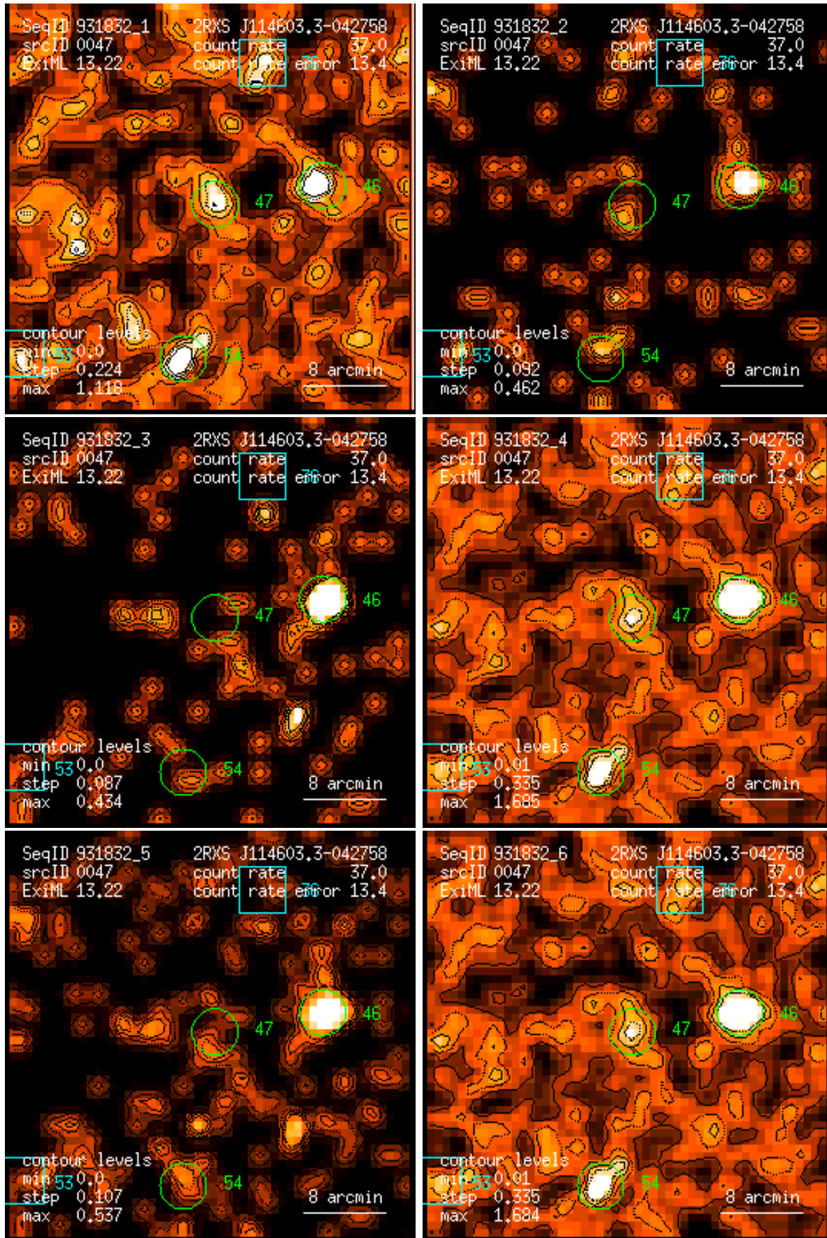
Figure 47: RASS 931832: detection 0047: band rate images, Gaussian filter: (1) PSPC channels 11 – 41, (2) 52 – 90, (3) 91 – 201, (4) 11 – 235, (5) 52 – 201, (6) 11 – 201. Broad band rates in counts/ks. Band rate contour levels in counts/ks/arcmin 2 .
