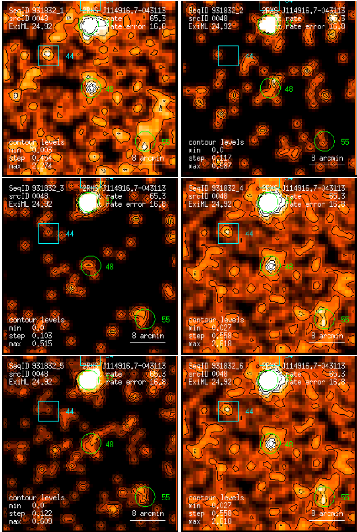
Figure 48: RASS 931832: detection 0048: band rate images, Gaussian filter: (1) PSPC channels 11 – 41, (2) 52 – 90, (3) 91 – 201, (4) 11 – 235, (5) 52 – 201, (6) 11 – 201. Broad band rates in counts/ks. Band rate contour levels in counts/ks/arcmin 2 .
