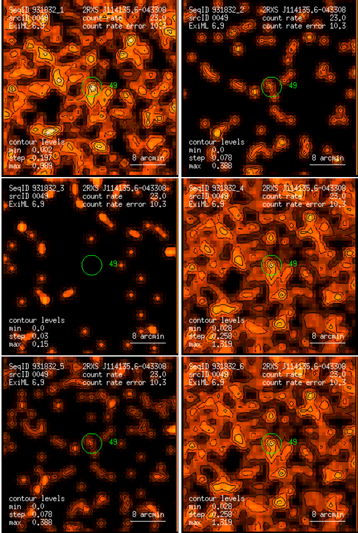
Figure 49: RASS 931832: detection 0049: band rate images, Gaussian filter: (1) PSPC channels 11 – 41, (2) 52 – 90, (3) 91 – 201, (4) 11 – 235, (5) 52 – 201, (6) 11 – 201. Broad band rates in counts/ks. Band rate contour levels in counts/ks/arcmin 2 .
