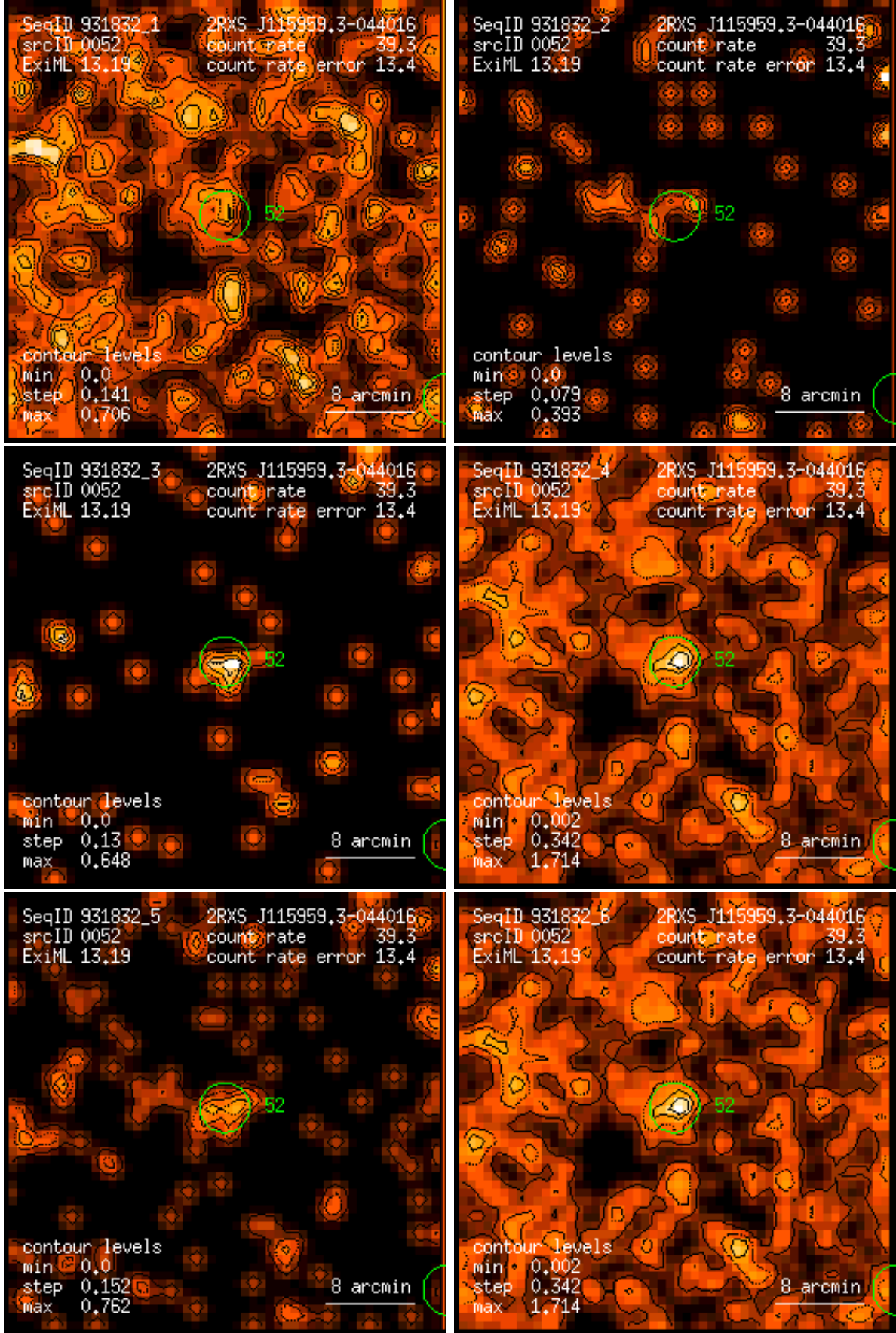
Figure 52: RASS 931832: detection 0052: band rate images, Gaussian filter: (1) PSPC channels 11 – 41, (2) 52 – 90, (3) 91 – 201, (4) 11 – 235, (5) 52 – 201, (6) 11 – 201. Broad band rates in counts/ks. Band rate contour levels in counts/ks/arcmin 2 .
