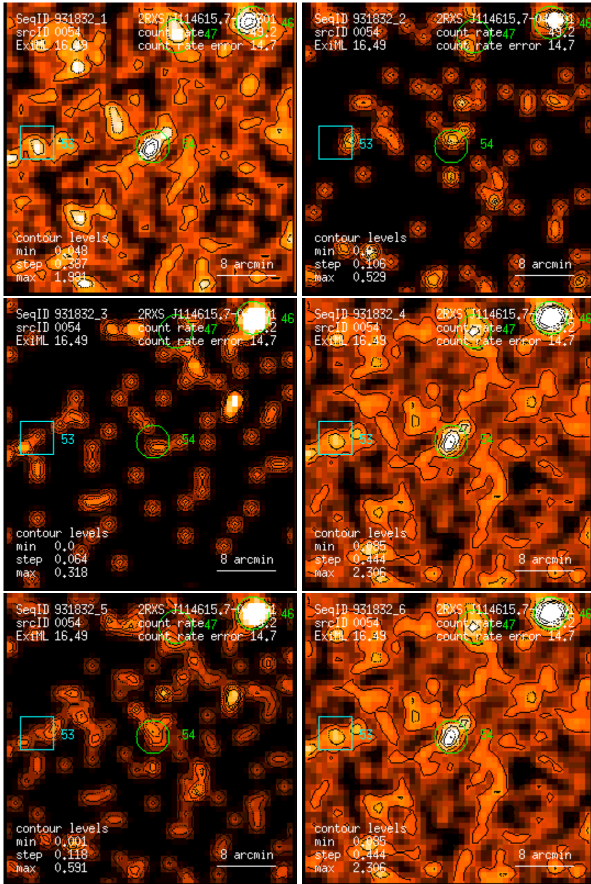
Figure 54: RASS 931832: detection 0054: band rate images, Gaussian filter: (1) PSPC channels 11 – 41, (2) 52 – 90, (3) 91 – 201, (4) 11 – 235, (5) 52 – 201, (6) 11 – 201. Broad band rates in counts/ks. Band rate contour levels in counts/ks/arcmin 2 .
