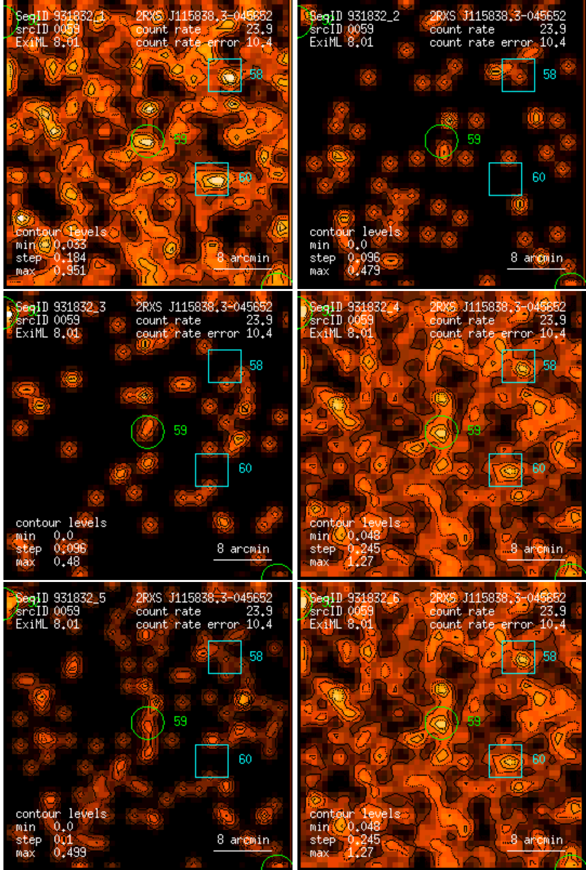
Figure 59: RASS 931832: detection 0059: band rate images, Gaussian filter: (1) PSPC channels 11 – 41, (2) 52 – 90, (3) 91 – 201, (4) 11 – 235, (5) 52 – 201, (6) 11 – 201. Broad band rates in counts/ks. Band rate contour levels in counts/ks/arcmin 2 .
