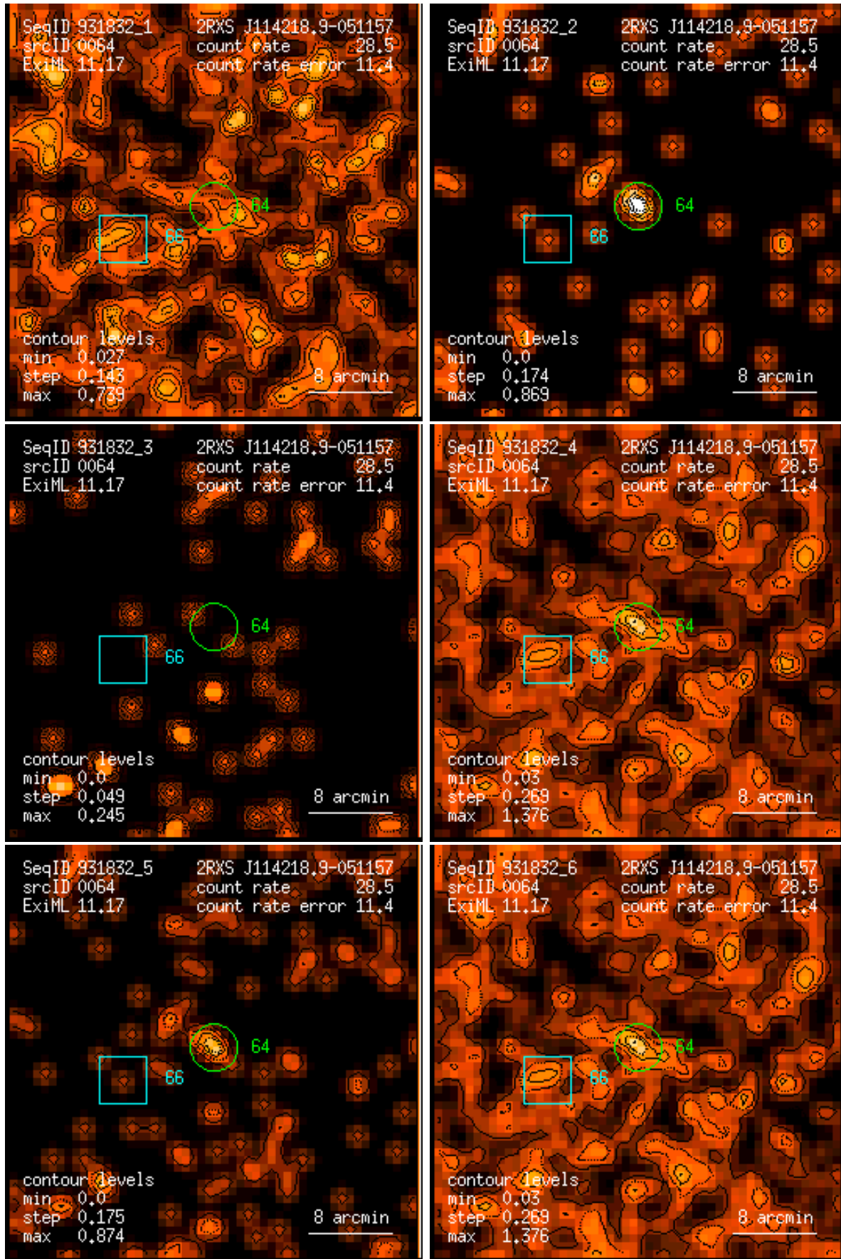
Figure 64: RASS 931832: detection 0064: band rate images, Gaussian filter: (1) PSPC channels 11 – 41, (2) 52 – 90, (3) 91 – 201, (4) 11 – 235, (5) 52 – 201, (6) 11 – 201. Broad band rates in counts/ks. Band rate contour levels in counts/ks/arcmin 2 .
