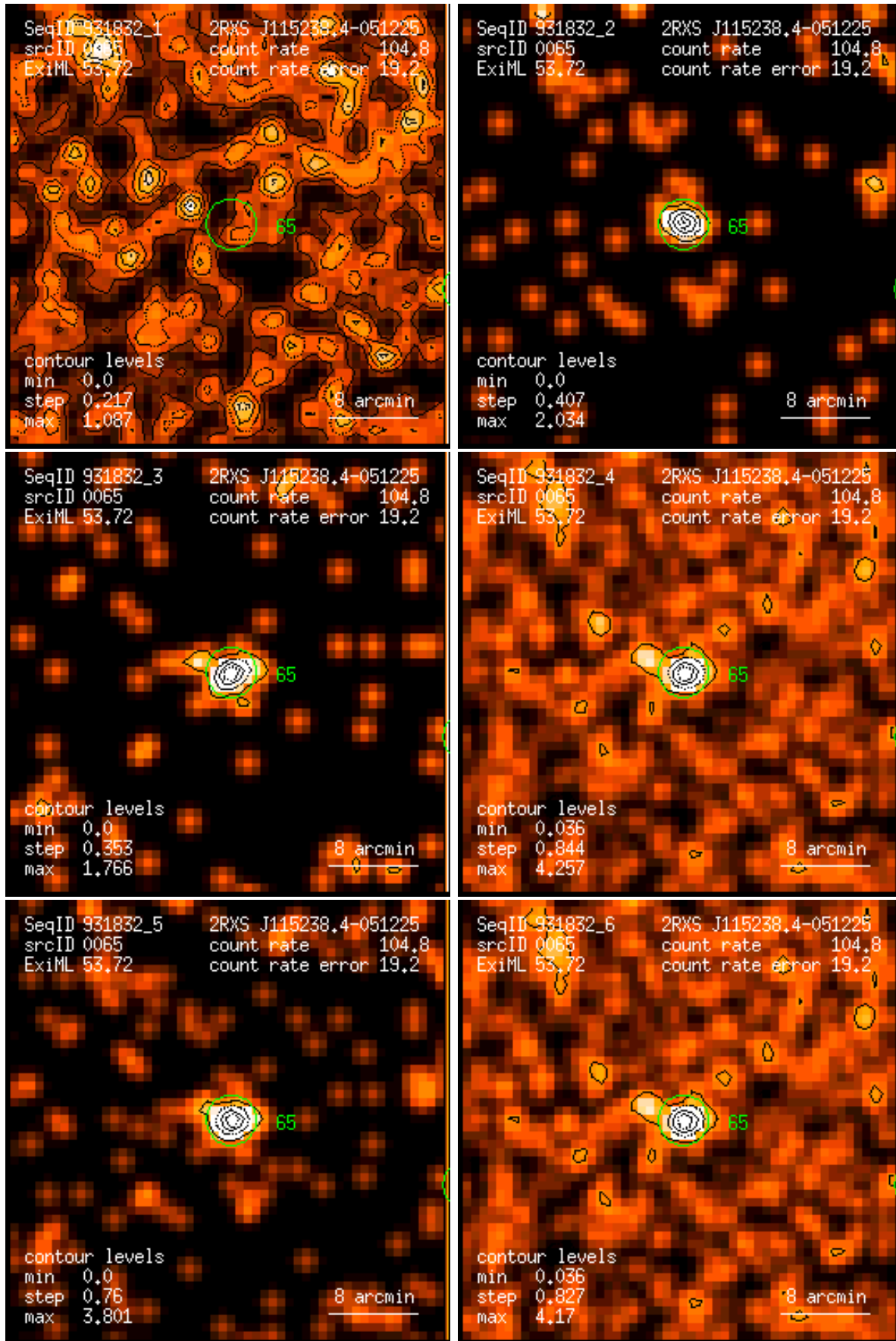
Figure 65: RASS 931832: detection 0065: band rate images, Gaussian filter: (1) PSPC channels 11 – 41, (2) 52 – 90, (3) 91 – 201, (4) 11 – 235, (5) 52 – 201, (6) 11 – 201. Broad band rates in counts/ks. Band rate contour levels in counts/ks/arcmin 2 .
