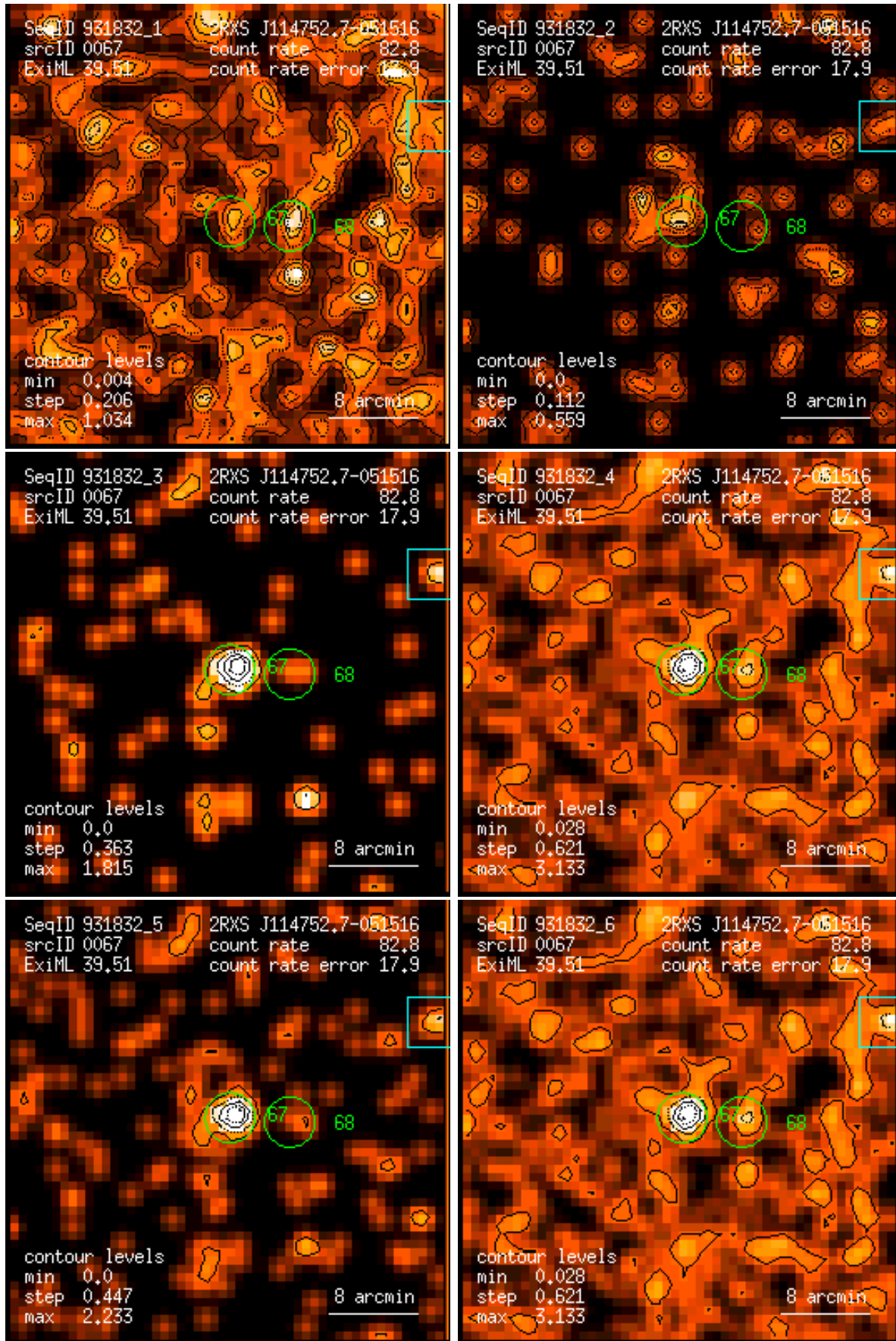
Figure 67: RASS 931832: detection 0067: band rate images, Gaussian filter: (1) PSPC channels 11 – 41, (2) 52 – 90, (3) 91 – 201, (4) 11 – 235, (5) 52 – 201, (6) 11 – 201. Broad band rates in counts/ks. Band rate contour levels in counts/ks/arcmin 2 .
