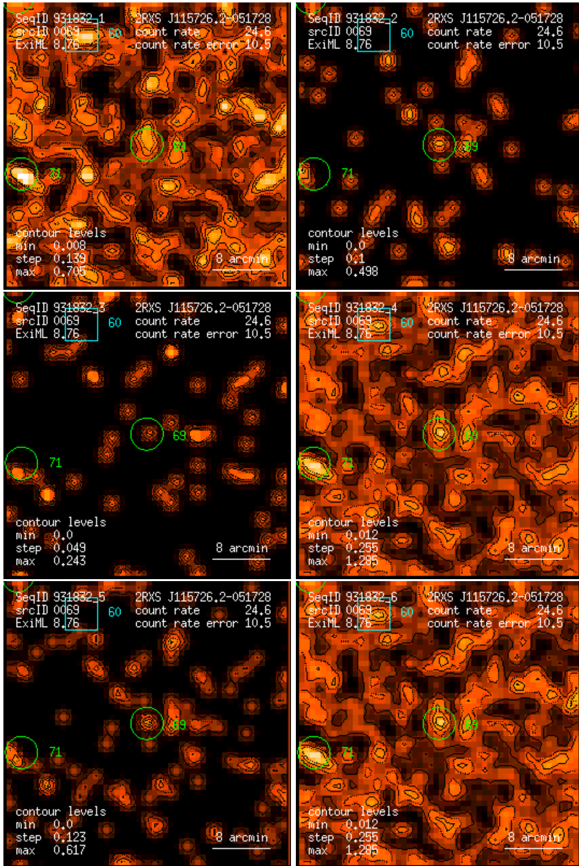
Figure 69: RASS 931832: detection 0069: band rate images, Gaussian filter: (1) PSPC channels 11 – 41, (2) 52 – 90, (3) 91 – 201, (4) 11 – 235, (5) 52 – 201, (6) 11 – 201. Broad band rates in counts/ks. Band rate contour levels in counts/ks/arcmin 2 .
