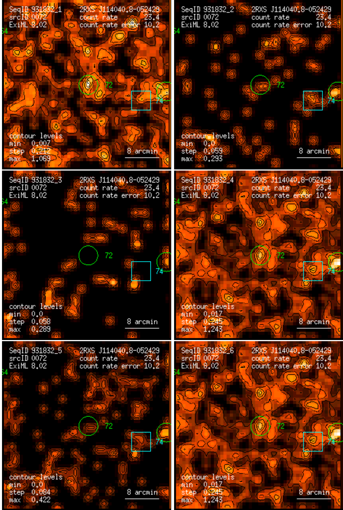
Figure 72: RASS 931832: detection 0072: band rate images, Gaussian filter: (1) PSPC channels 11 – 41, (2) 52 – 90, (3) 91 – 201, (4) 11 – 235, (5) 52 – 201, (6) 11 – 201. Broad band rates in counts/ks. Band rate contour levels in counts/ks/arcmin 2 .
