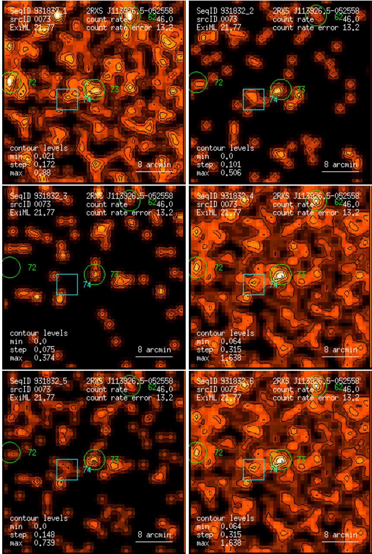
Figure 73: RASS 931832: detection 0073: band rate images, Gaussian filter: (1) PSPC channels 11 – 41, (2) 52 – 90, (3) 91 – 201, (4) 11 – 235, (5) 52 – 201, (6) 11 – 201. Broad band rates in counts/ks. Band rate contour levels in counts/ks/arcmin 2 .
