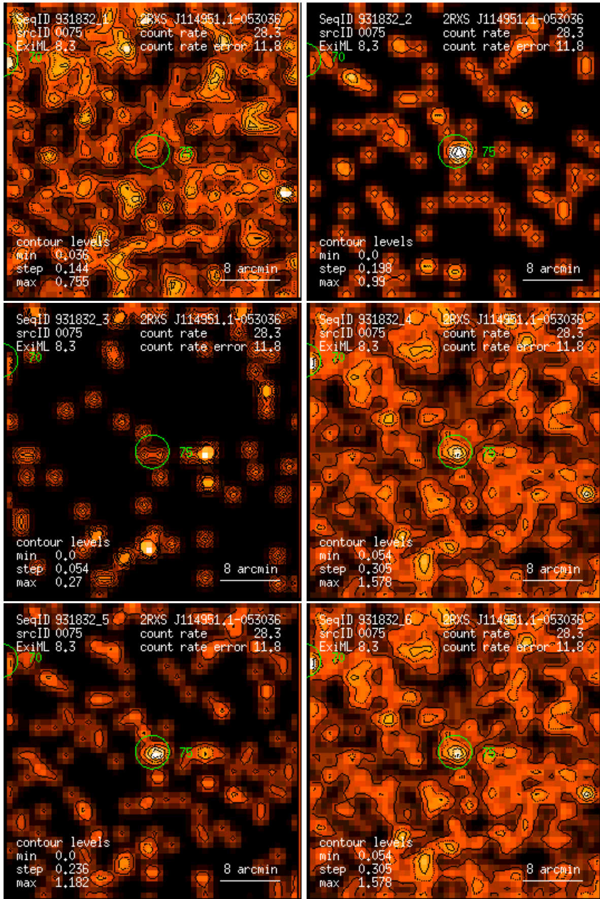
Figure 75: RASS 931832: detection 0075: band rate images, Gaussian filter: (1) PSPC channels 11 – 41, (2) 52 – 90, (3) 91 – 201, (4) 11 – 235, (5) 52 – 201, (6) 11 – 201. Broad band rates in counts/ks. Band rate contour levels in counts/ks/arcmin 2 .
