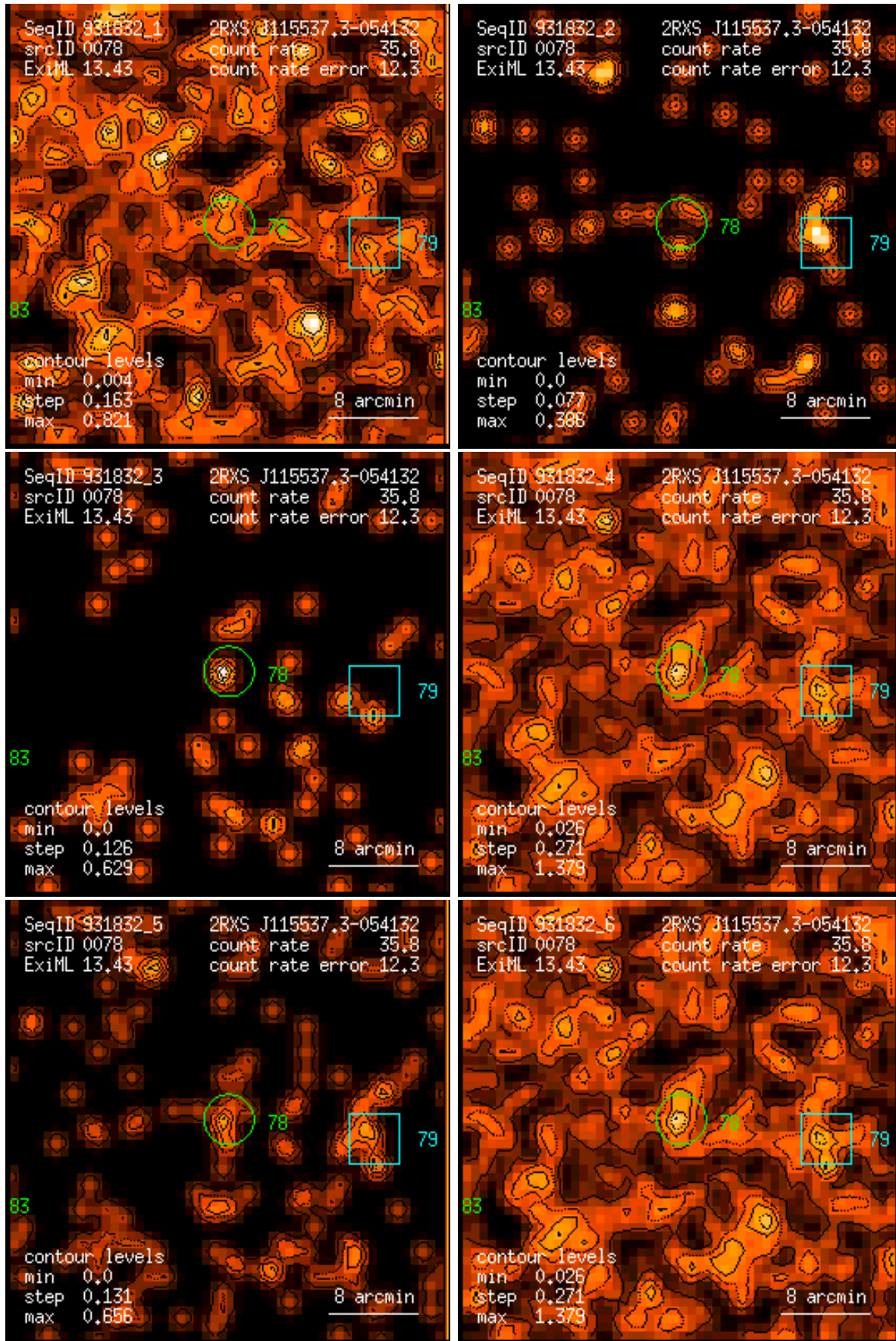
Figure 78: RASS 931832: detection 0078: band rate images, Gaussian filter: (1) PSPC channels 11 – 41, (2) 52 – 90, (3) 91 – 201, (4) 11 – 235, (5) 52 – 201, (6) 11 – 201. Broad band rates in counts/ks. Band rate contour levels in counts/ks/arcmin 2 .
