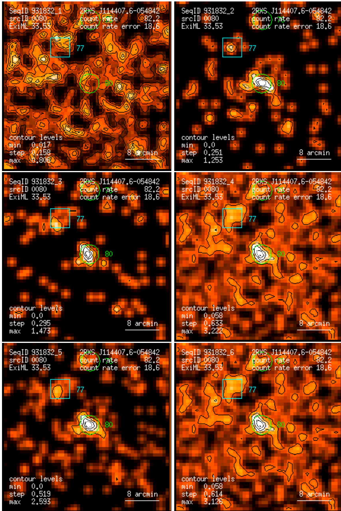
Figure 80: RASS 931832: detection 0080: band rate images, Gaussian filter: (1) PSPC channels 11 – 41, (2) 52 – 90, (3) 91 – 201, (4) 11 – 235, (5) 52 – 201, (6) 11 – 201. Broad band rates in counts/ks. Band rate contour levels in counts/ks/arcmin 2 .
