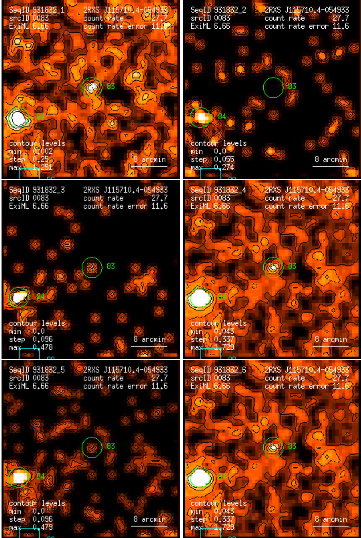
Figure 83: RASS 931832: detection 0083: band rate images, Gaussian filter: (1) PSPC channels 11 – 41, (2) 52 – 90, (3) 91 – 201, (4) 11 – 235, (5) 52 – 201, (6) 11 – 201. Broad band rates in counts/ks. Band rate contour levels in counts/ks/arcmin 2 .
