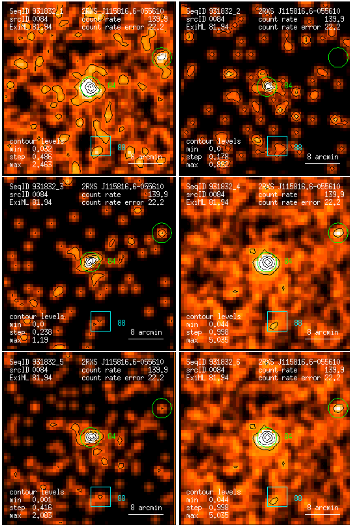
Figure 84: RASS 931832: detection 0084: band rate images, Gaussian filter: (1) PSPC channels 11 – 41, (2) 52 – 90, (3) 91 – 201, (4) 11 – 235, (5) 52 – 201, (6) 11 – 201. Broad band rates in counts/ks. Band rate contour levels in counts/ks/arcmin 2 .
