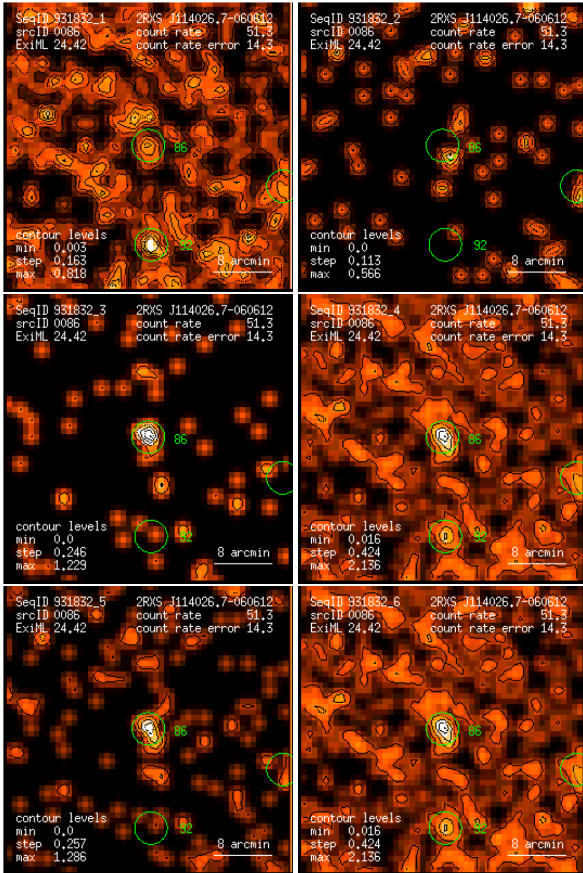
Figure 86: RASS 931832: detection 0086: band rate images, Gaussian filter: (1) PSPC channels 11 – 41, (2) 52 – 90, (3) 91 – 201, (4) 11 – 235, (5) 52 – 201, (6) 11 – 201. Broad band rates in counts/ks. Band rate contour levels in counts/ks/arcmin 2 .
