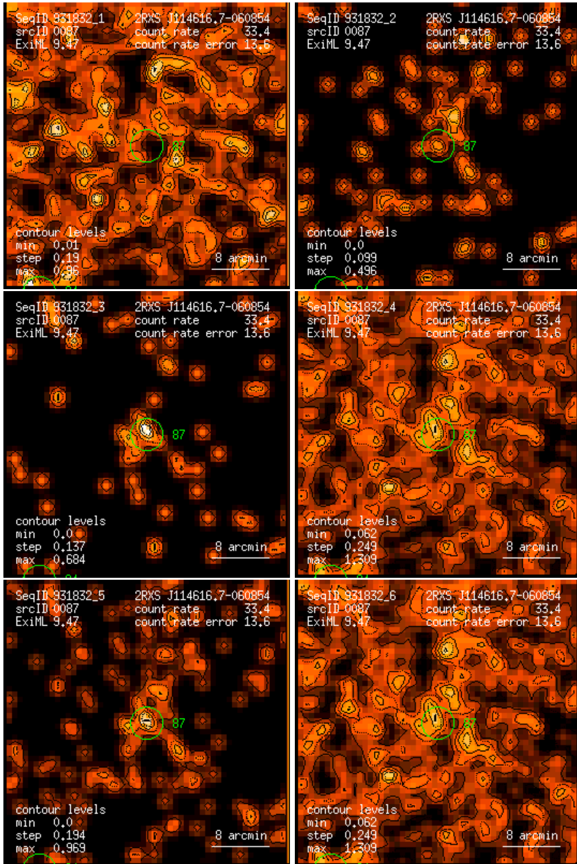
Figure 87: RASS 931832: detection 0087: band rate images, Gaussian filter: (1) PSPC channels 11 – 41, (2) 52 – 90, (3) 91 – 201, (4) 11 – 235, (5) 52 – 201, (6) 11 – 201. Broad band rates in counts/ks. Band rate contour levels in counts/ks/arcmin 2 .
