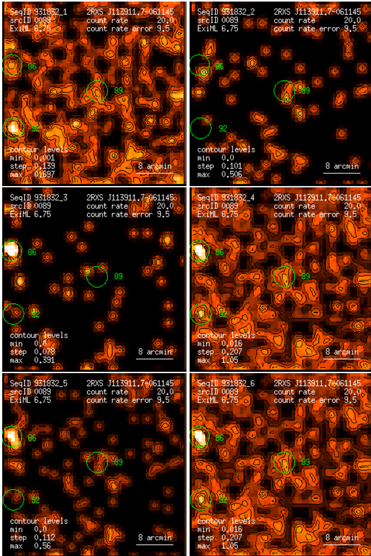
Figure 89: RASS 931832: detection 0089: band rate images, Gaussian filter: (1) PSPC channels 11 – 41, (2) 52 – 90, (3) 91 – 201, (4) 11 – 235, (5) 52 – 201, (6) 11 – 201. Broad band rates in counts/ks. Band rate contour levels in counts/ks/arcmin 2 .
