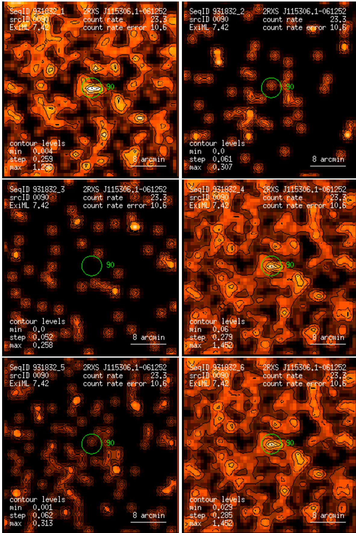
Figure 90: RASS 931832: detection 0090: band rate images, Gaussian filter: (1) PSPC channels 11 – 41, (2) 52 – 90, (3) 91 – 201, (4) 11 – 235, (5) 52 – 201, (6) 11 – 201. Broad band rates in counts/ks. Band rate contour levels in counts/ks/arcmin 2 .
