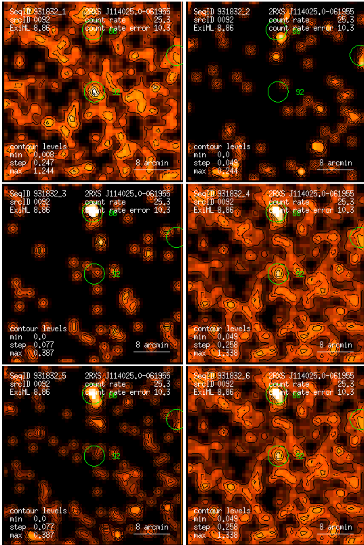
Figure 92: RASS 931832: detection 0092: band rate images, Gaussian filter: (1) PSPC channels 11 – 41, (2) 52 – 90, (3) 91 – 201, (4) 11 – 235, (5) 52 – 201, (6) 11 – 201. Broad band rates in counts/ks. Band rate contour levels in counts/ks/arcmin 2 .
