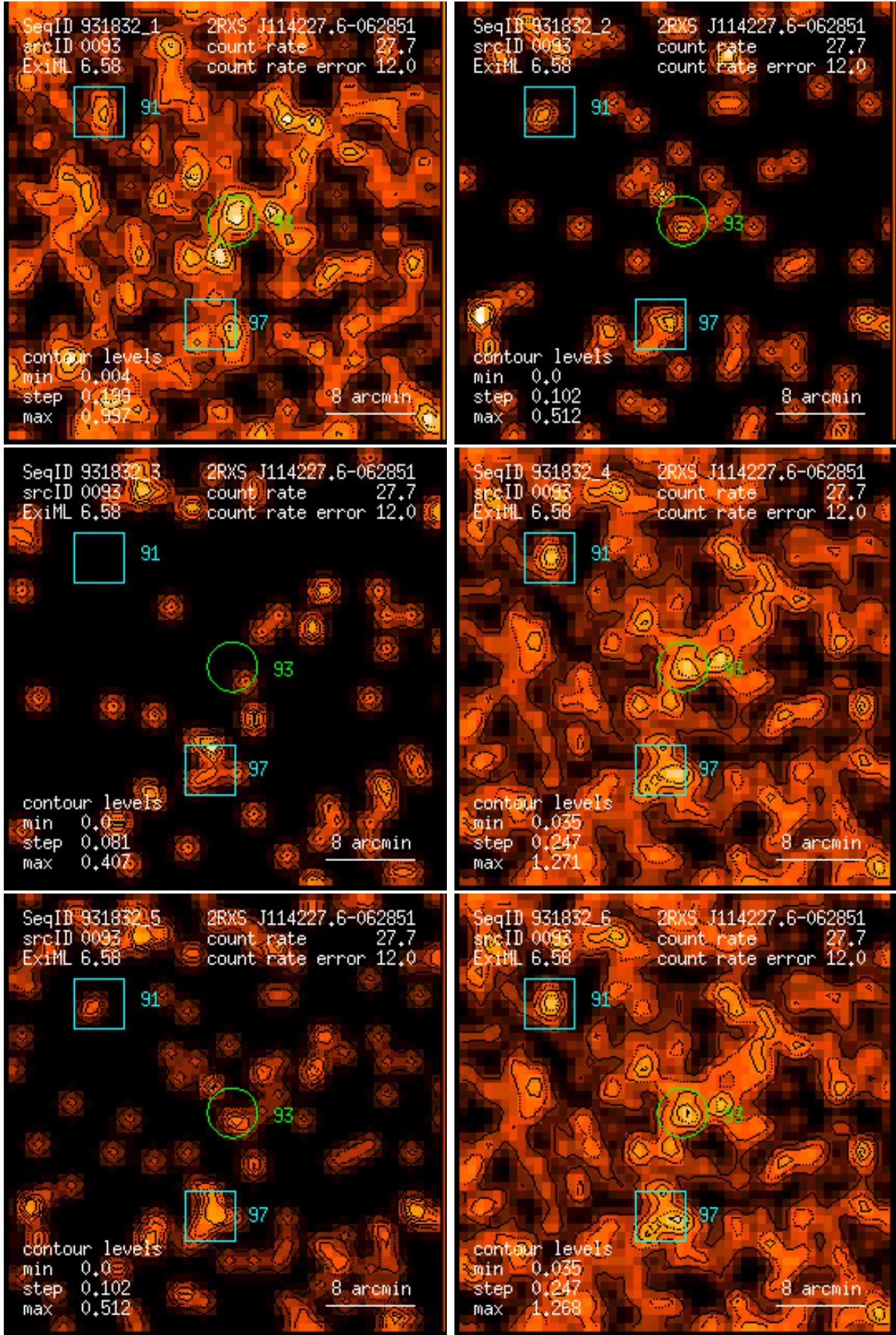
Figure 93: RASS 931832: detection 0093: band rate images, Gaussian filter: (1) PSPC channels 11 – 41, (2) 52 – 90, (3) 91 – 201, (4) 11 – 235, (5) 52 – 201, (6) 11 – 201. Broad band rates in counts/ks. Band rate contour levels in counts/ks/arcmin 2 .
