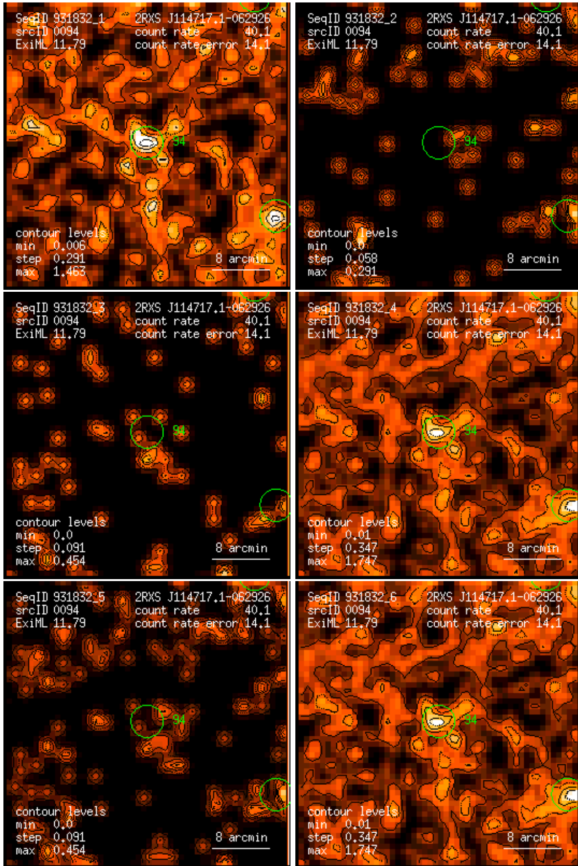
Figure 94: RASS 931832: detection 0094: band rate images, Gaussian filter: (1) PSPC channels 11 – 41, (2) 52 – 90, (3) 91 – 201, (4) 11 – 235, (5) 52 – 201, (6) 11 – 201. Broad band rates in counts/ks. Band rate contour levels in counts/ks/arcmin 2 .
