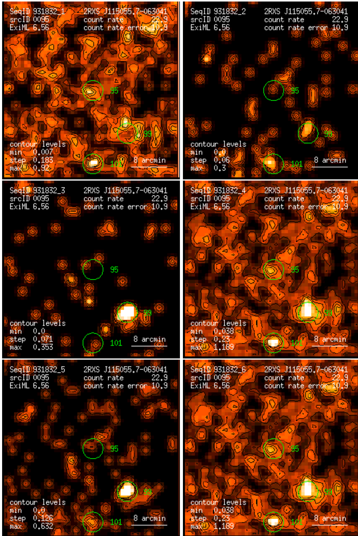
Figure 95: RASS 931832: detection 0095: band rate images, Gaussian filter: (1) PSPC channels 11 – 41, (2) 52 – 90, (3) 91 – 201, (4) 11 – 235, (5) 52 – 201, (6) 11 – 201. Broad band rates in counts/ks. Band rate contour levels in counts/ks/arcmin 2 .
