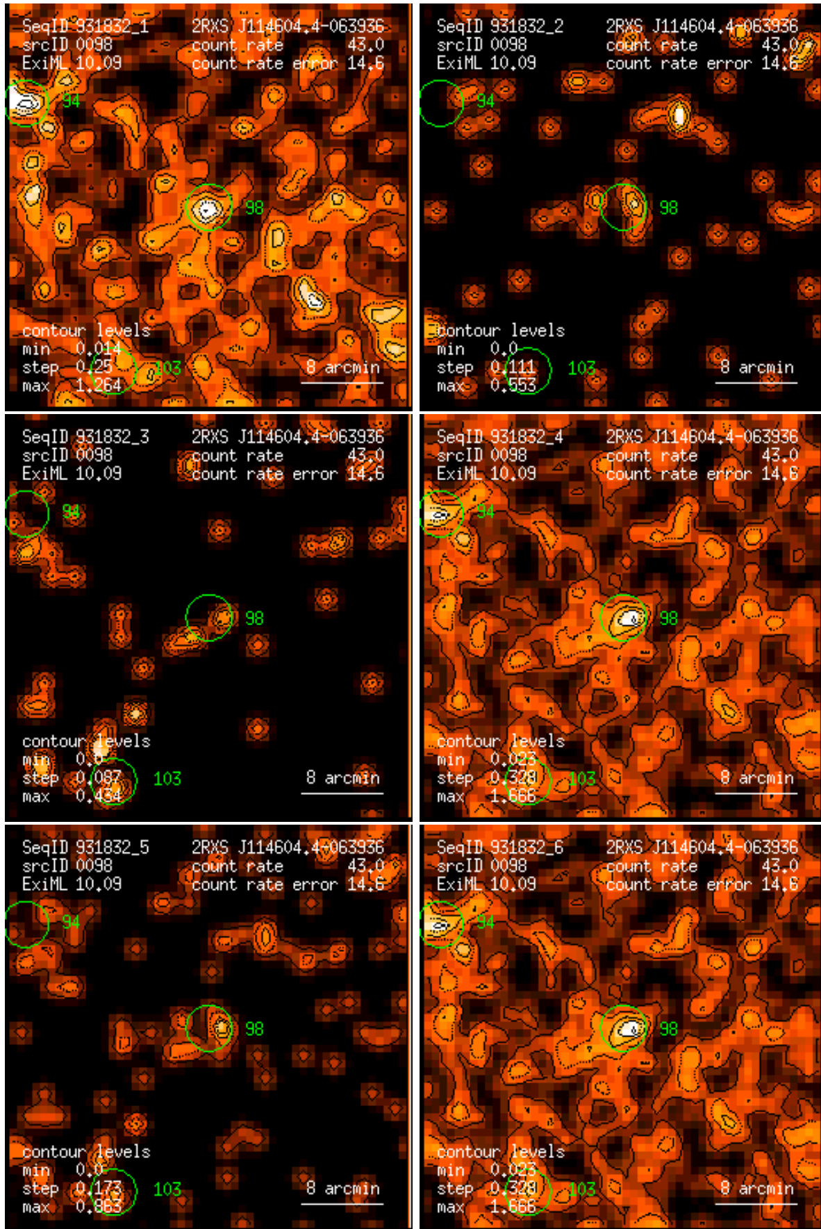
Figure 98: RASS 931832: detection 0098: band rate images, Gaussian filter: (1) PSPC channels 11 – 41, (2) 52 – 90, (3) 91 – 201, (4) 11 – 235, (5) 52 – 201, (6) 11 – 201. Broad band rates in counts/ks. Band rate contour levels in counts/ks/arcmin 2 .
