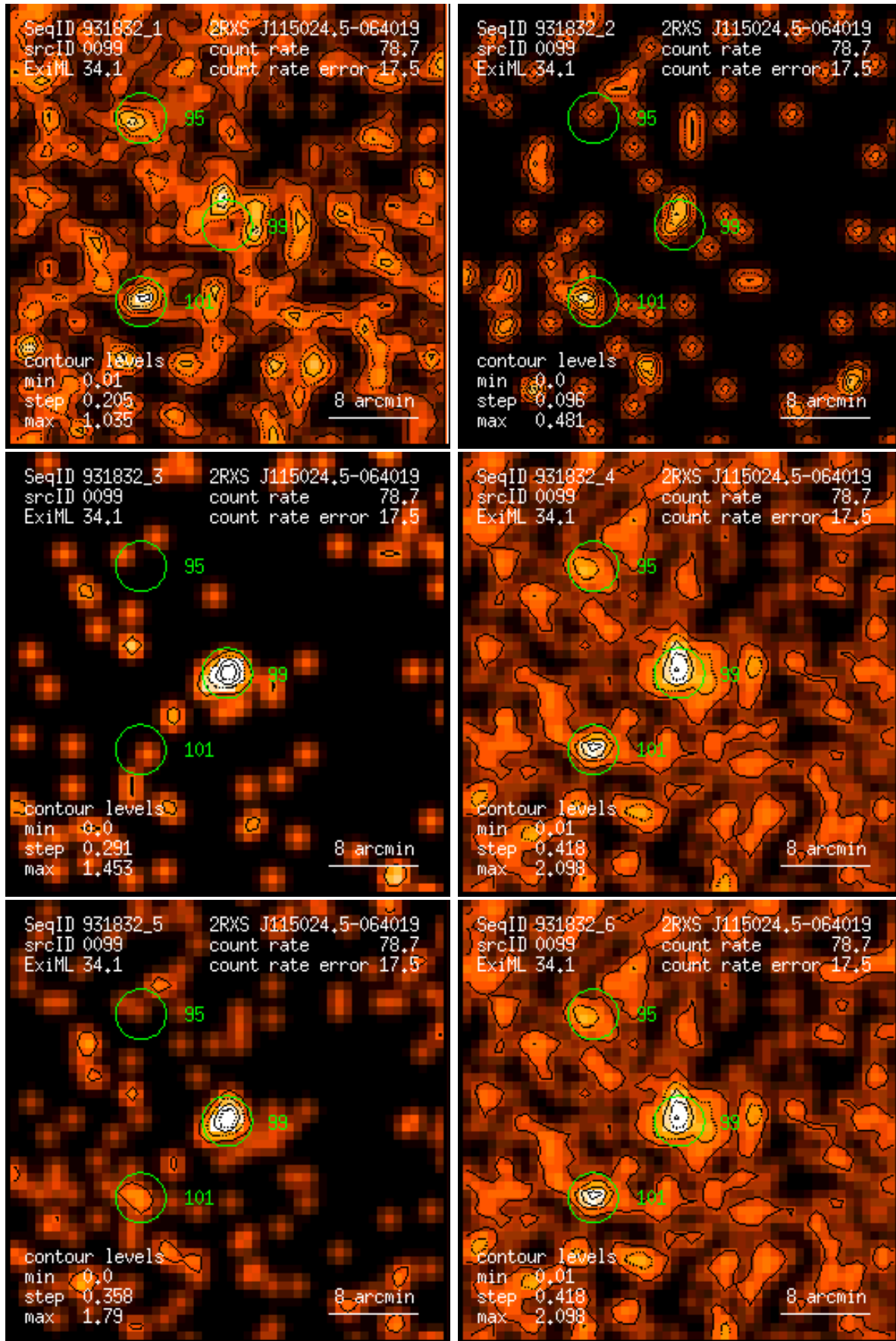
Figure 99: RASS 931832: detection 0099: band rate images, Gaussian filter: (1) PSPC channels 11 – 41, (2) 52 – 90, (3) 91 – 201, (4) 11 – 235, (5) 52 – 201, (6) 11 – 201. Broad band rates in counts/ks. Band rate contour levels in counts/ks/arcmin 2 .
