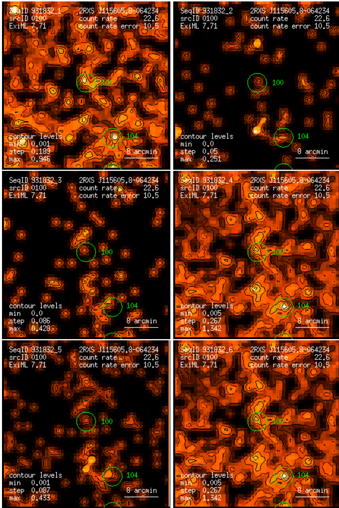
Figure 100: RASS 931832: detection 0100: band rate images, Gaussian filter: (1) PSPC channels 11 – 41, (2) 52 – 90, (3) 91 – 201, (4) 11 – 235, (5) 52 – 201, (6) 11 – 201. Broad band rates in counts/ks. Band rate contour levels in counts/ks/arcmin 2 .
