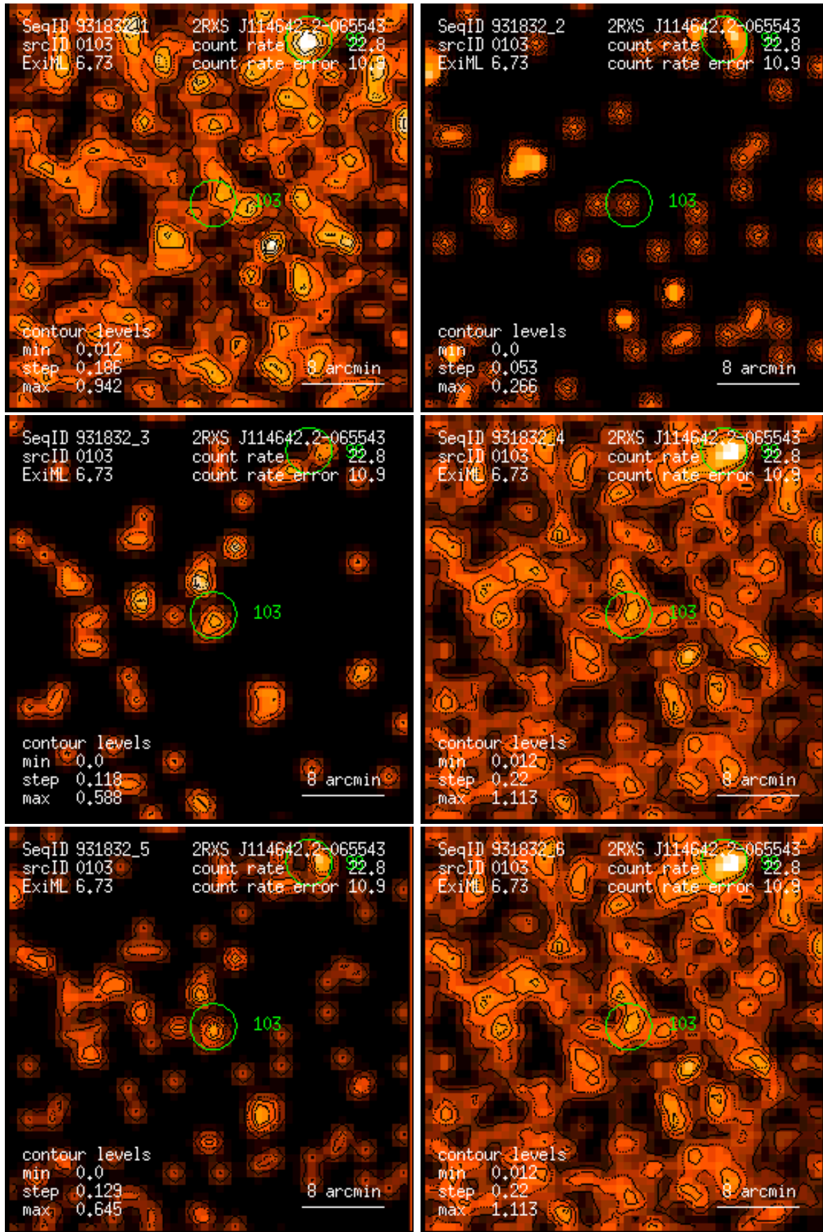
Figure 103: RASS 931832: detection 0103: band rate images, Gaussian filter: (1) PSPC channels 11 – 41, (2) 52 – 90, (3) 91 – 201, (4) 11 – 235, (5) 52 – 201, (6) 11 – 201. Broad band rates in counts/ks. Band rate contour levels in counts/ks/arcmin 2 .
