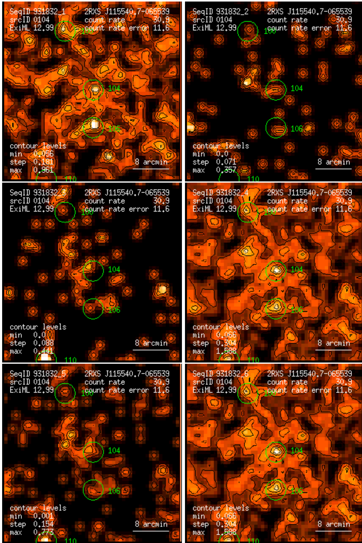
Figure 104: RASS 931832: detection 0104: band rate images, Gaussian filter: (1) PSPC channels 11 – 41, (2) 52 – 90, (3) 91 – 201, (4) 11 – 235, (5) 52 – 201, (6) 11 – 201. Broad band rates in counts/ks. Band rate contour levels in counts/ks/arcmin 2 .
