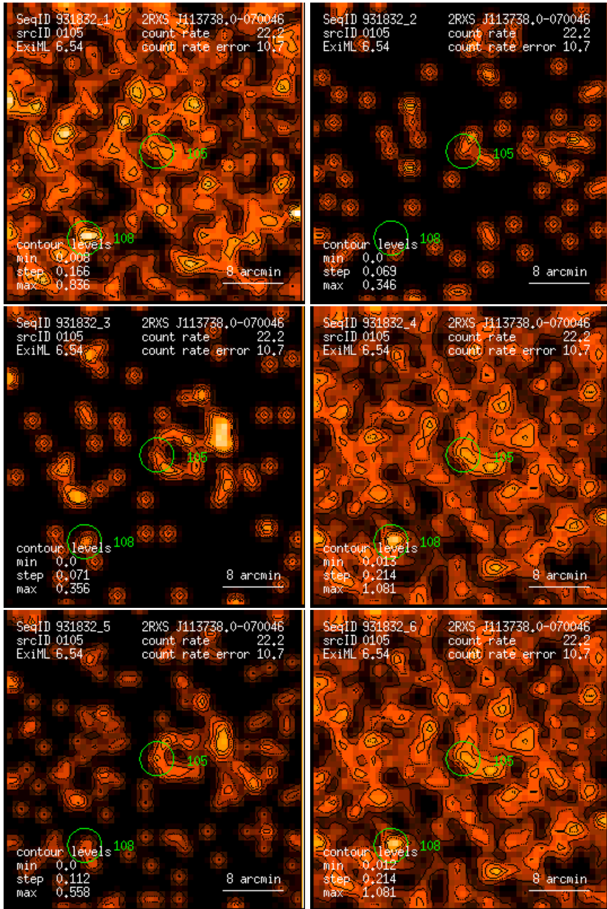
Figure 105: RASS 931832: detection 0105: band rate images, Gaussian filter: (1) PSPC channels 11 – 41, (2) 52 – 90, (3) 91 – 201, (4) 11 – 235, (5) 52 – 201, (6) 11 – 201. Broad band rates in counts/ks. Band rate contour levels in counts/ks/arcmin 2 .
