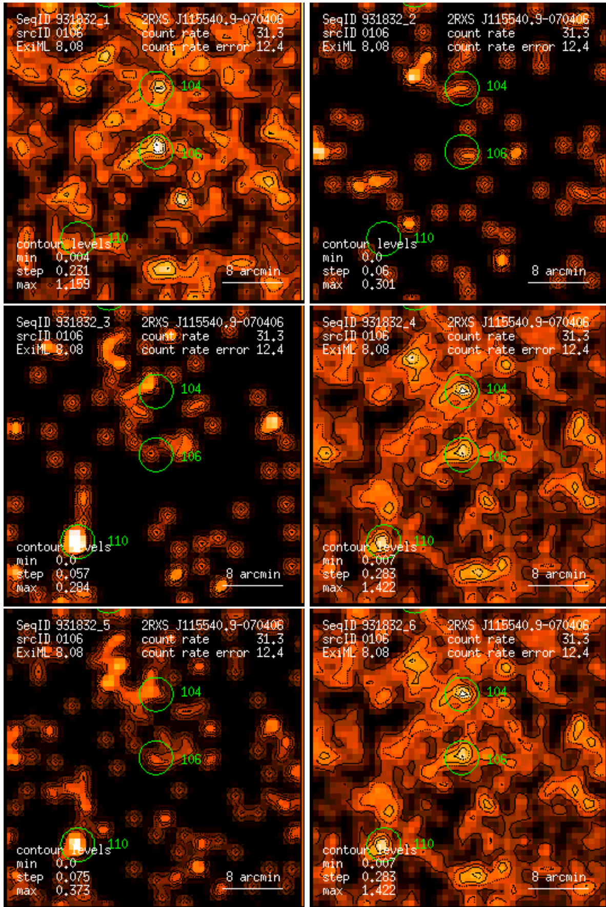
Figure 106: RASS 931832: detection 0106: band rate images, Gaussian filter: (1) PSPC channels 11 – 41, (2) 52 – 90, (3) 91 – 201, (4) 11 – 235, (5) 52 – 201, (6) 11 – 201. Broad band rates in counts/ks. Band rate contour levels in counts/ks/arcmin 2 .
