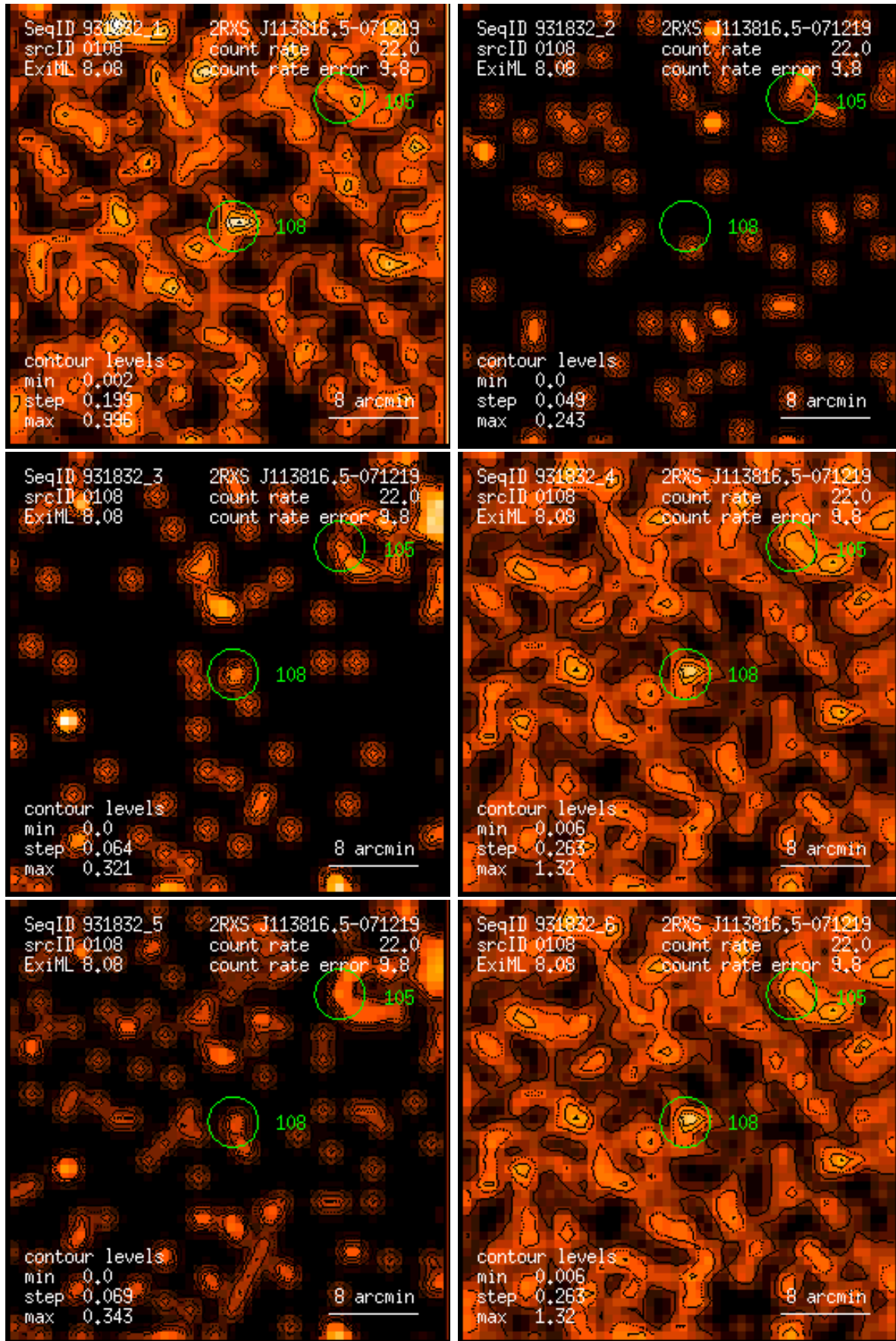
Figure 108: RASS 931832: detection 0108: band rate images, Gaussian filter: (1) PSPC channels 11 – 41, (2) 52 – 90, (3) 91 – 201, (4) 11 – 235, (5) 52 – 201, (6) 11 – 201. Broad band rates in counts/ks. Band rate contour levels in counts/ks/arcmin 2 .
