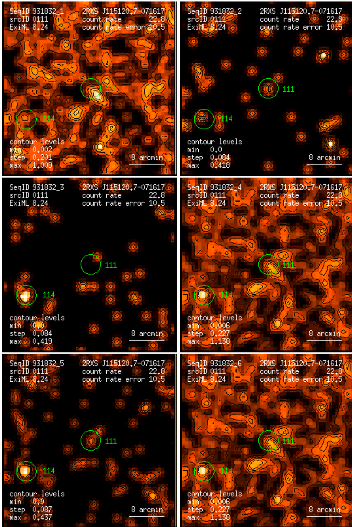
Figure 111: RASS 931832: detection 0111: band rate images, Gaussian filter: (1) PSPC channels 11 – 41, (2) 52 – 90, (3) 91 – 201, (4) 11 – 235, (5) 52 – 201, (6) 11 – 201. Broad band rates in counts/ks. Band rate contour levels in counts/ks/arcmin 2 .
