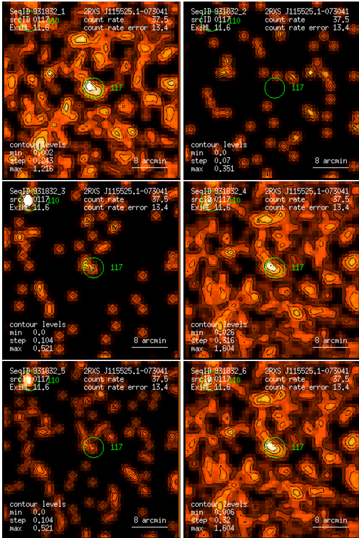
Figure 117: RASS 931832: detection 0117: band rate images, Gaussian filter: (1) PSPC channels 11 – 41, (2) 52 – 90, (3) 91 – 201, (4) 11 – 235, (5) 52 – 201, (6) 11 – 201. Broad band rates in counts/ks. Band rate contour levels in counts/ks/arcmin 2 .
