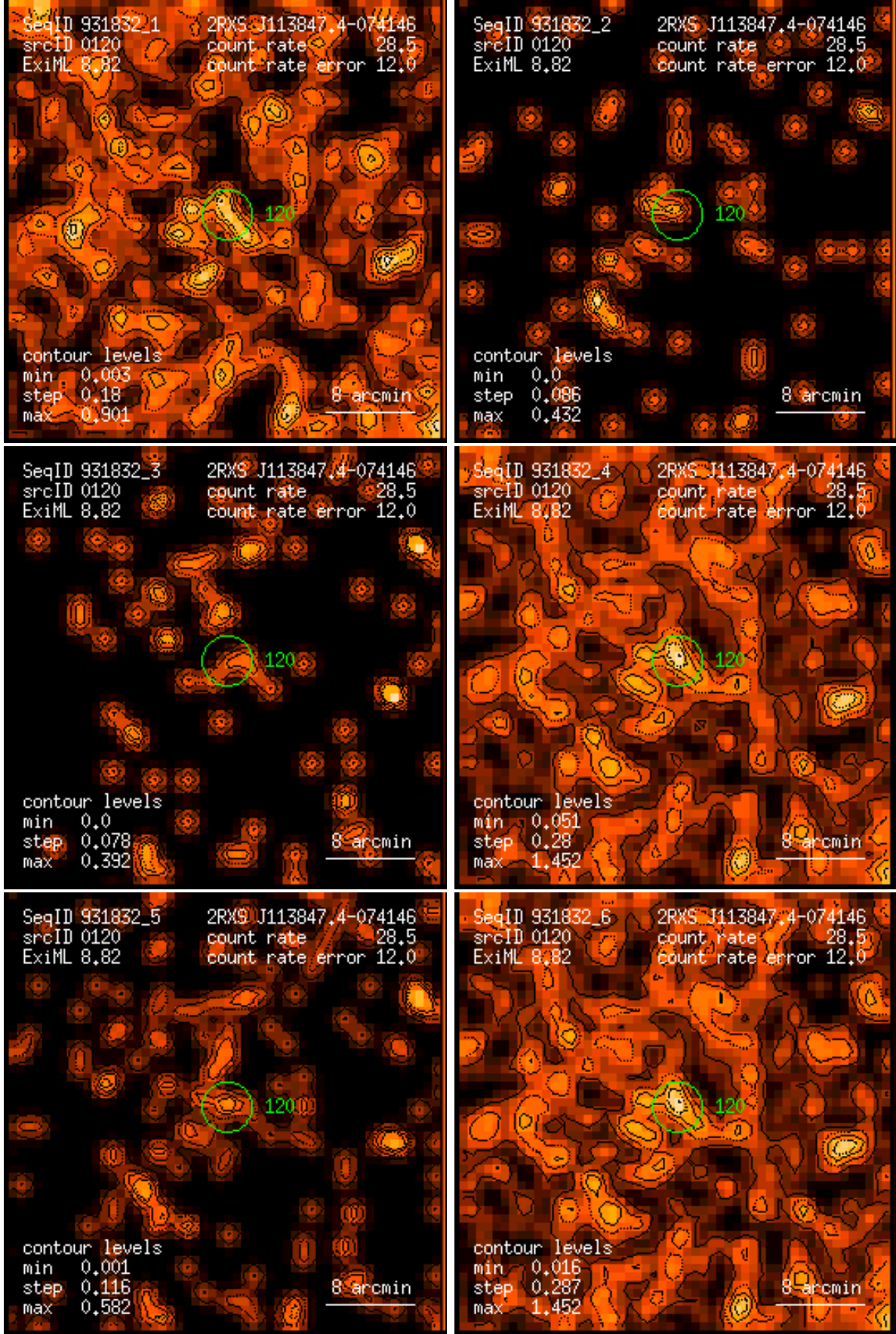
Figure 120: RASS 931832: detection 0120: band rate images, Gaussian filter: (1) PSPC channels 11 – 41, (2) 52 – 90, (3) 91 – 201, (4) 11 – 235, (5) 52 – 201, (6) 11 – 201. Broad band rates in counts/ks. Band rate contour levels in counts/ks/arcmin 2 .
