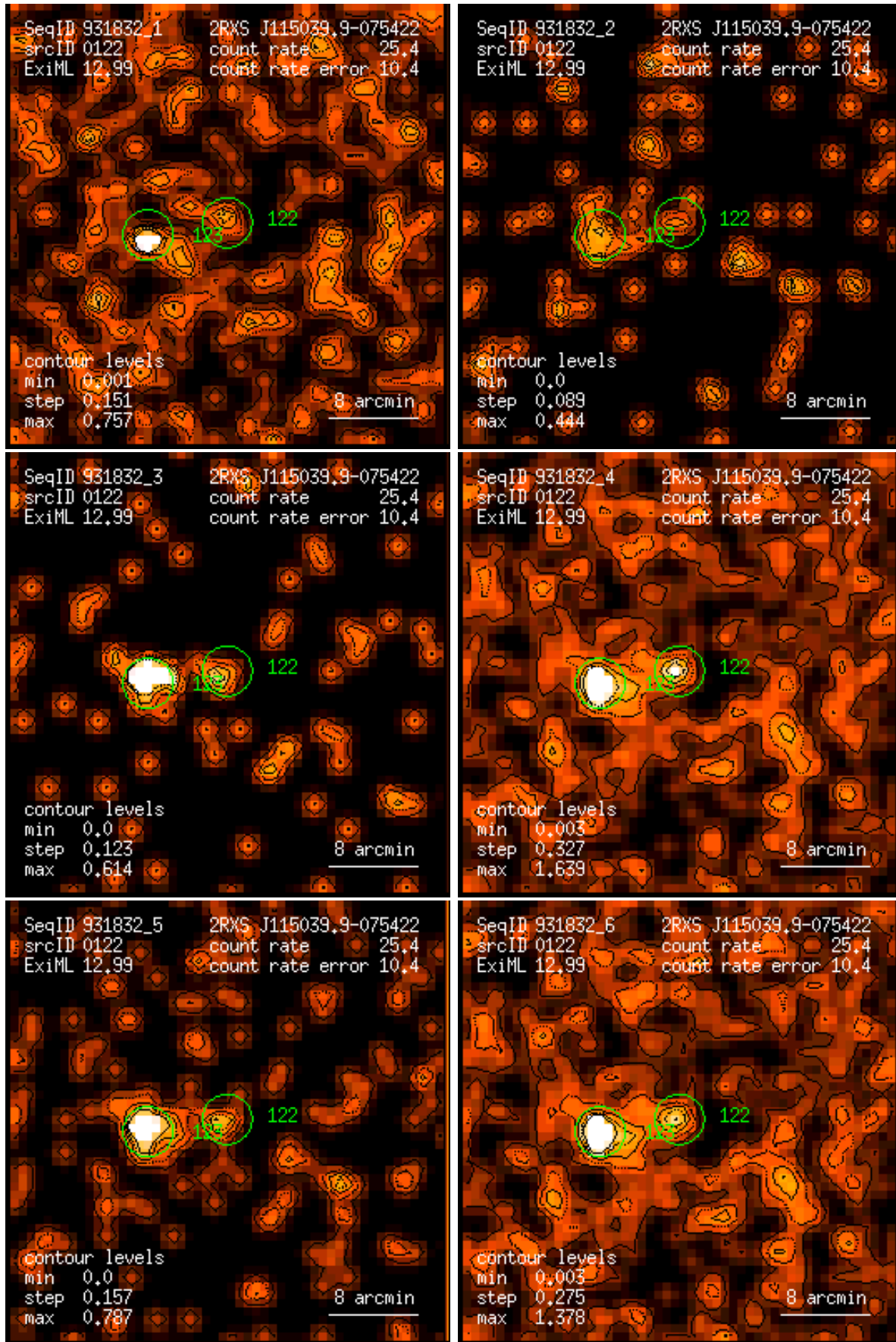
Figure 122: RASS 931832: detection 0122: band rate images, Gaussian filter: (1) PSPC channels 11 – 41, (2) 52 – 90, (3) 91 – 201, (4) 11 – 235, (5) 52 – 201, (6) 11 – 201. Broad band rates in counts/ks. Band rate contour levels in counts/ks/arcmin 2 .
