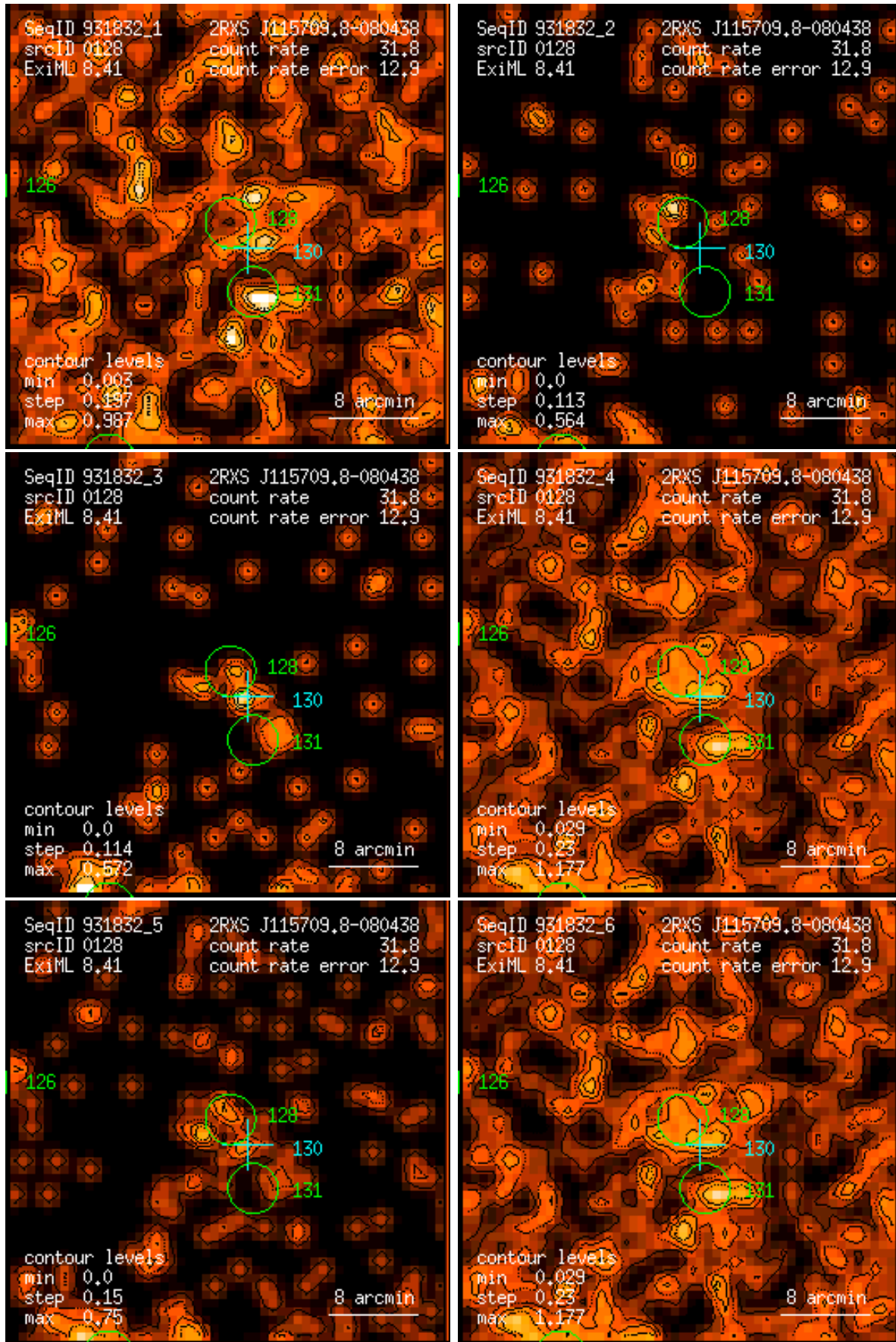
Figure 128: RASS 931832: detection 0128: band rate images, Gaussian filter: (1) PSPC channels 11 – 41, (2) 52 – 90, (3) 91 – 201, (4) 11 – 235, (5) 52 – 201, (6) 11 – 201. Broad band rates in counts/ks. Band rate contour levels in counts/ks/arcmin 2 .
