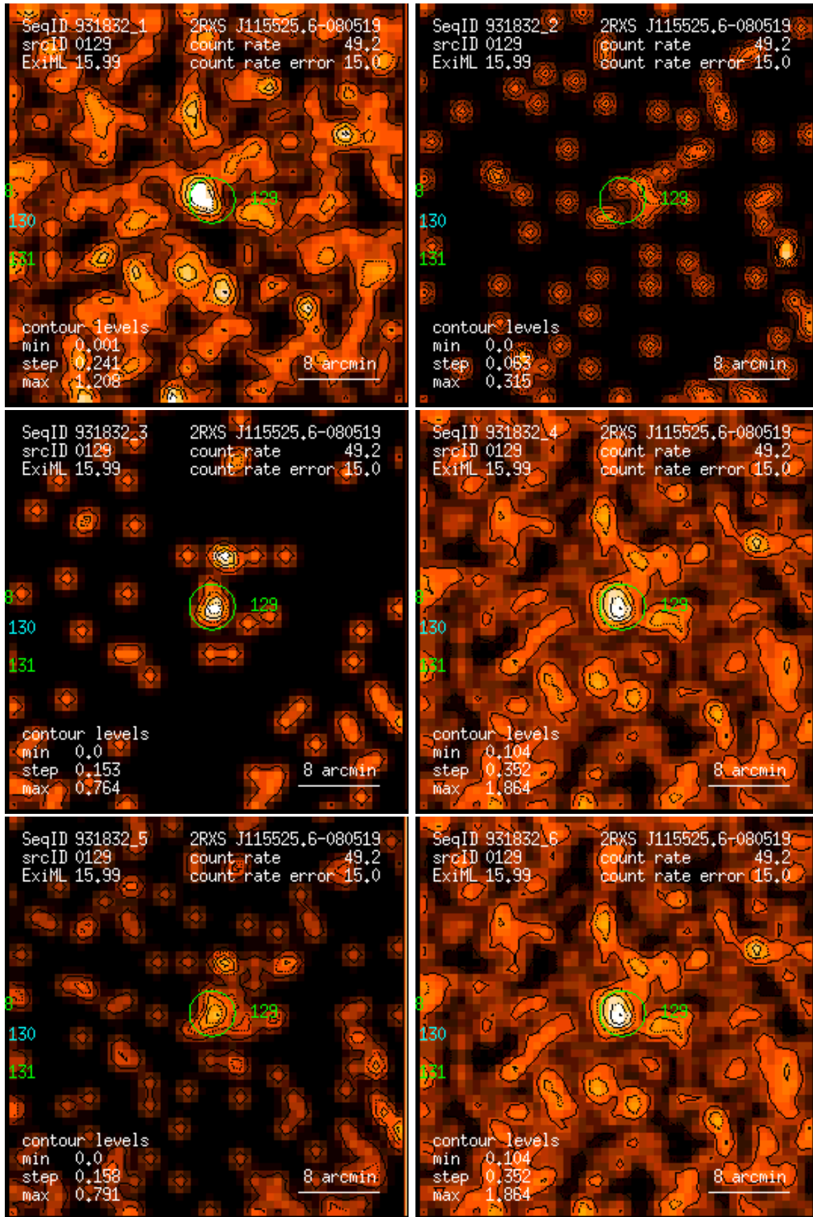
Figure 129: RASS 931832: detection 0129: band rate images, Gaussian filter: (1) PSPC channels 11 – 41, (2) 52 – 90, (3) 91 – 201, (4) 11 – 235, (5) 52 – 201, (6) 11 – 201. Broad band rates in counts/ks. Band rate contour levels in counts/ks/arcmin 2 .
