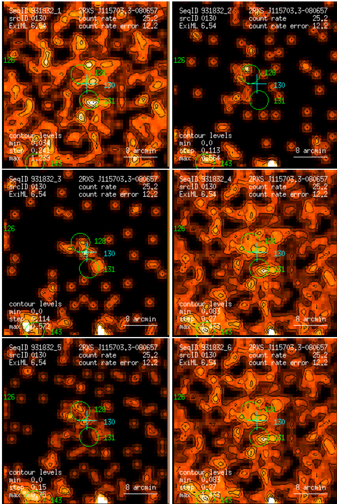
Figure 130: RASS 931832: detection 0130: band rate images, Gaussian filter: (1) PSPC channels 11 – 41, (2) 52 – 90, (3) 91 – 201, (4) 11 – 235, (5) 52 – 201, (6) 11 – 201. Broad band rates in counts/ks. Band rate contour levels in counts/ks/arcmin 2 .
