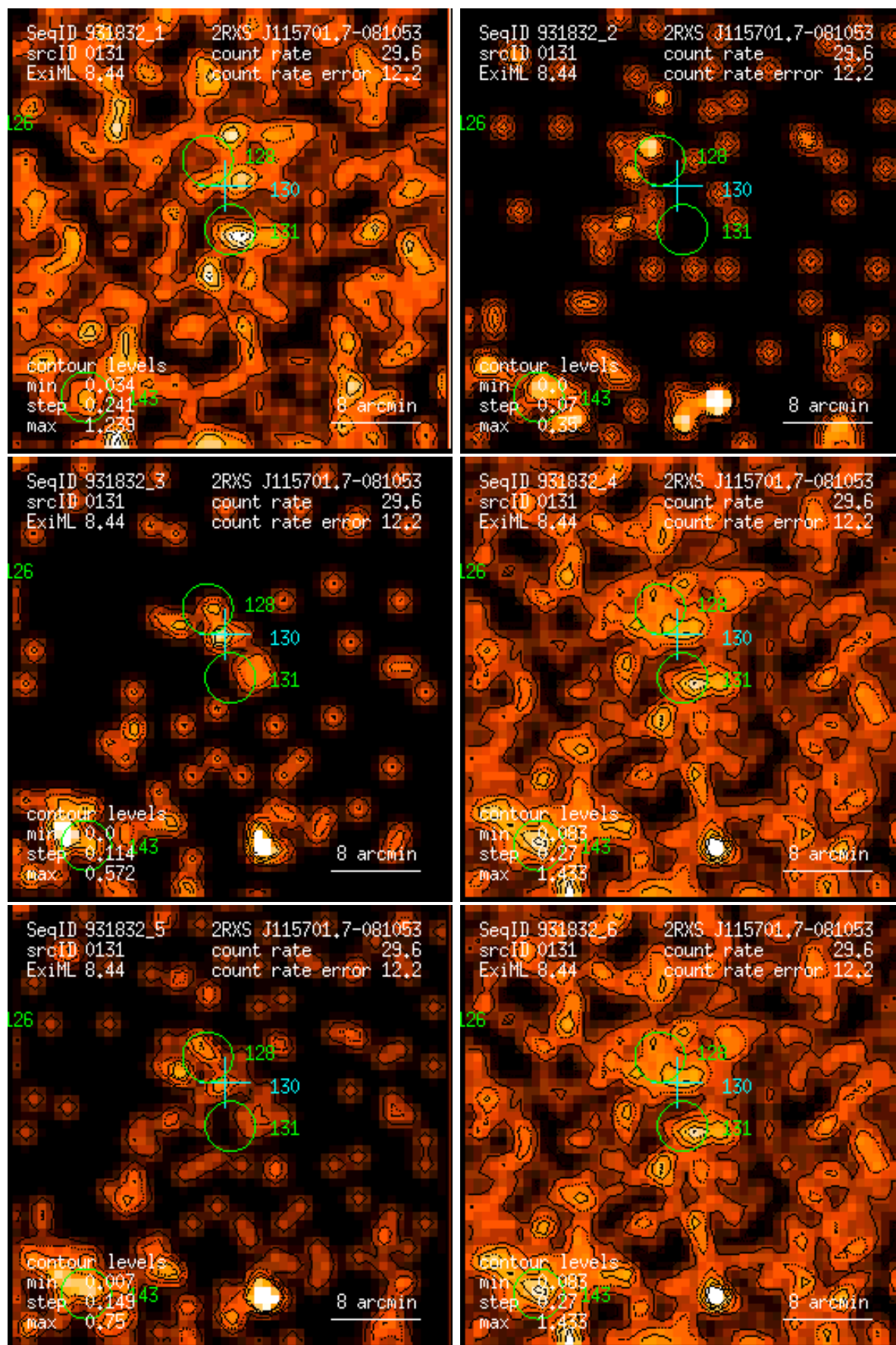
Figure 131: RASS 931832: detection 0131: band rate images, Gaussian filter: (1) PSPC channels 11 – 41, (2) 52 – 90, (3) 91 – 201, (4) 11 – 235, (5) 52 – 201, (6) 11 – 201. Broad band rates in counts/ks. Band rate contour levels in counts/ks/arcmin 2 .
