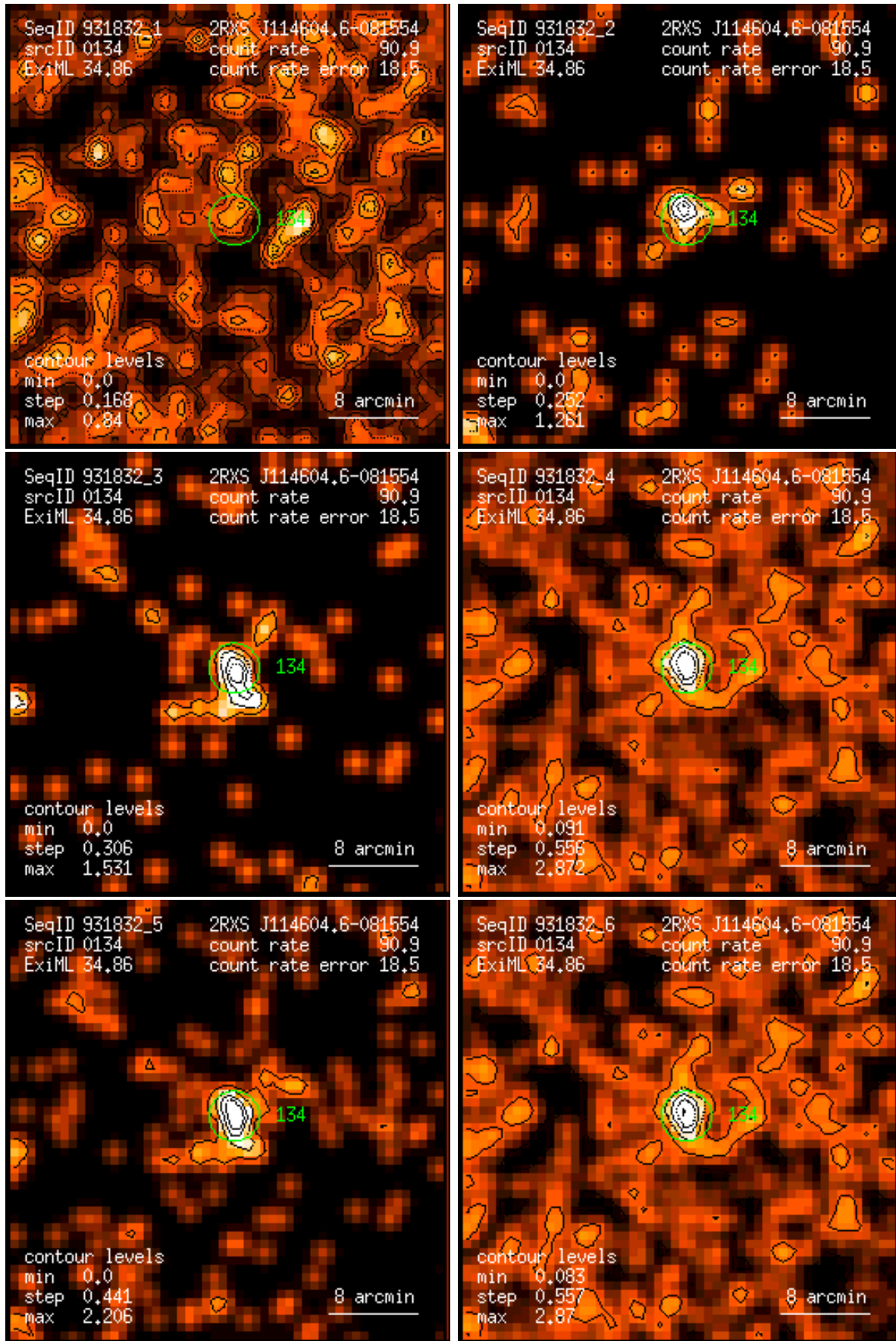
Figure 134: RASS 931832: detection 0134: band rate images, Gaussian filter: (1) PSPC channels 11 – 41, (2) 52 – 90, (3) 91 – 201, (4) 11 – 235, (5) 52 – 201, (6) 11 – 201. Broad band rates in counts/ks. Band rate contour levels in counts/ks/arcmin 2 .
