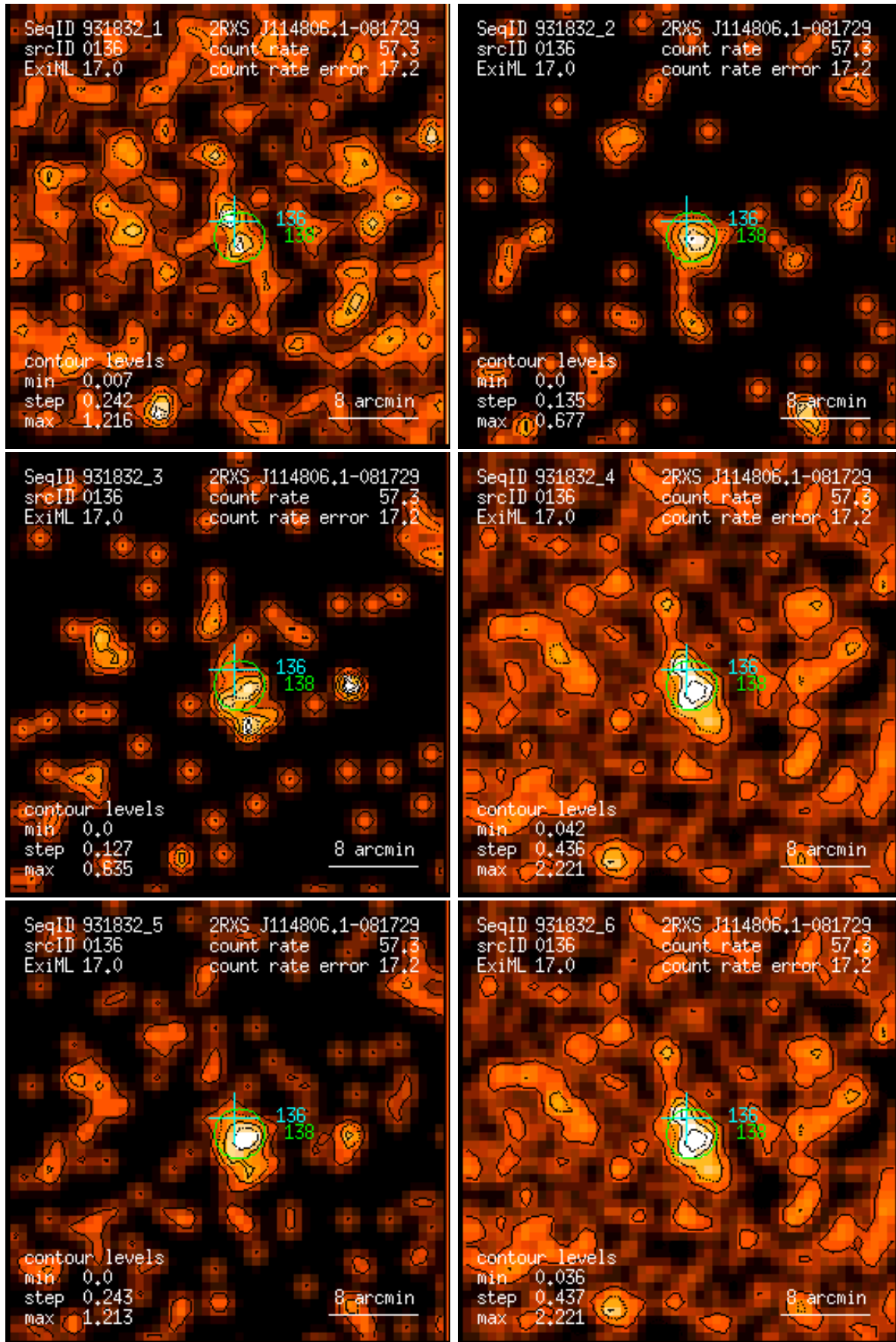
Figure 136: RASS 931832: detection 0136: band rate images, Gaussian filter: (1) PSPC channels 11 – 41, (2) 52 – 90, (3) 91 – 201, (4) 11 – 235, (5) 52 – 201, (6) 11 – 201. Broad band rates in counts/ks. Band rate contour levels in counts/ks/arcmin 2 .
