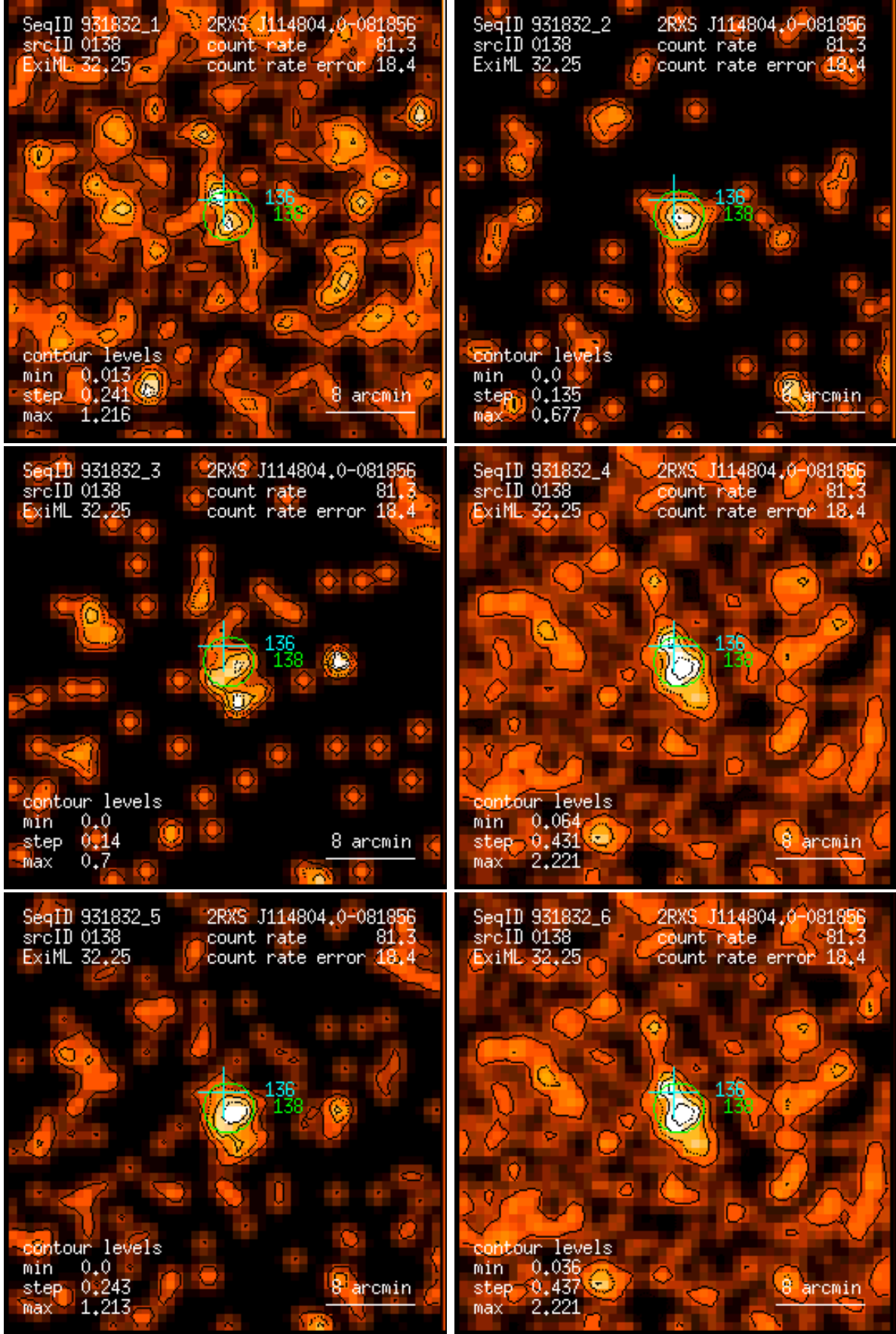
Figure 138: RASS 931832: detection 0138: band rate images, Gaussian filter: (1) PSPC channels 11 – 41, (2) 52 – 90, (3) 91 – 201, (4) 11 – 235, (5) 52 – 201, (6) 11 – 201. Broad band rates in counts/ks. Band rate contour levels in counts/ks/arcmin 2 .
